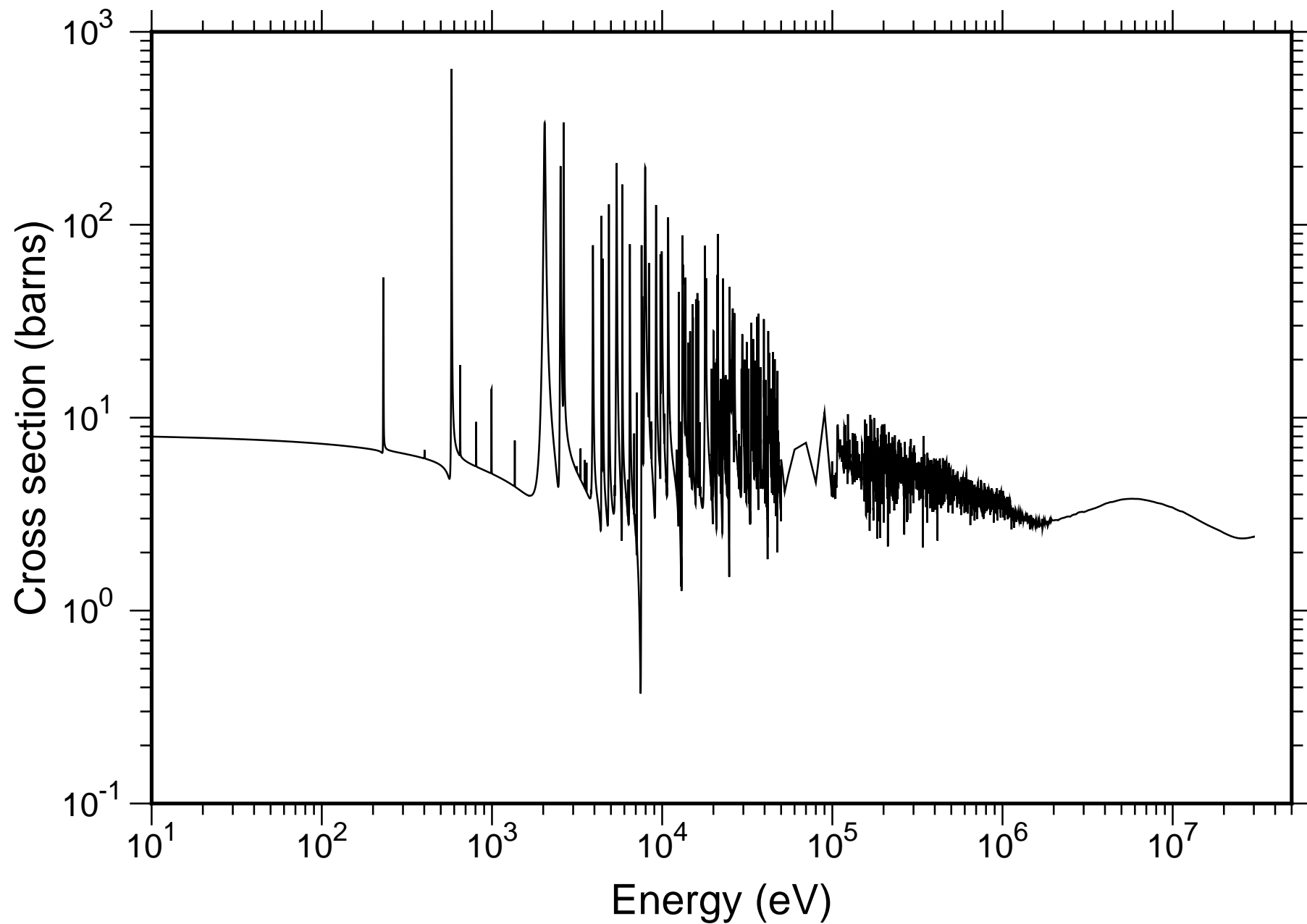
Natural Cu Total Cross-section - TENDL-2019
