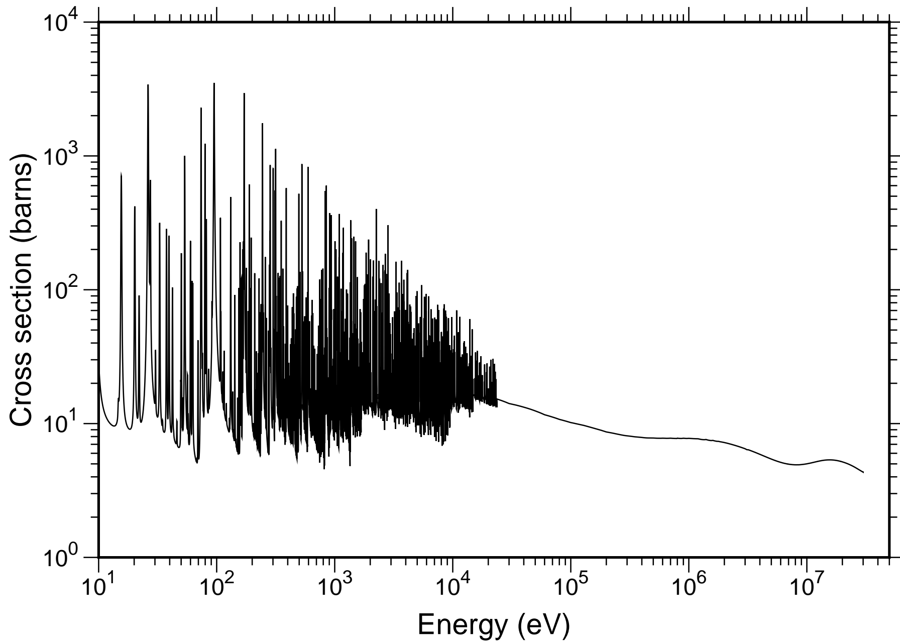
Natural Er Total Cross-section - TENDL-2019
