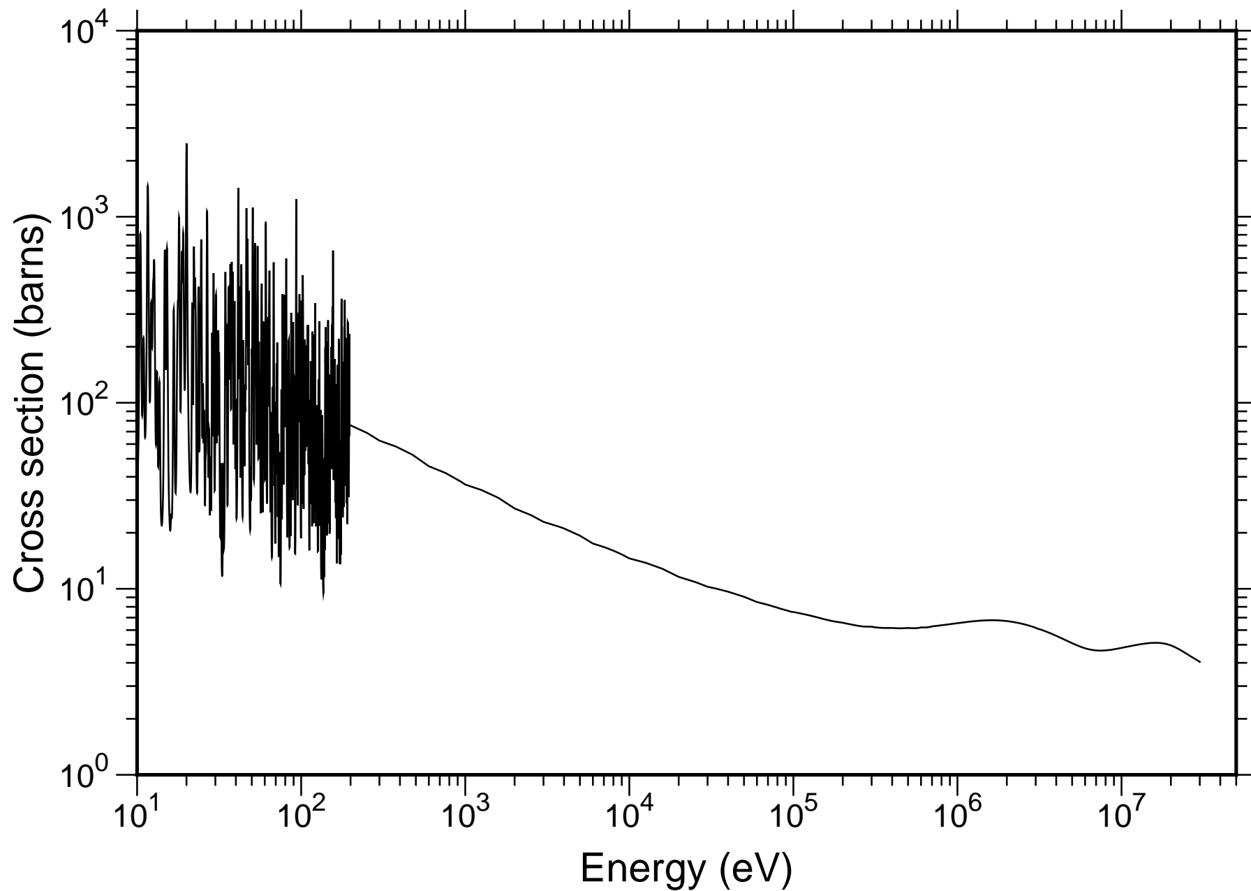
Natural Eu Total Cross-section - TENDL-2019
