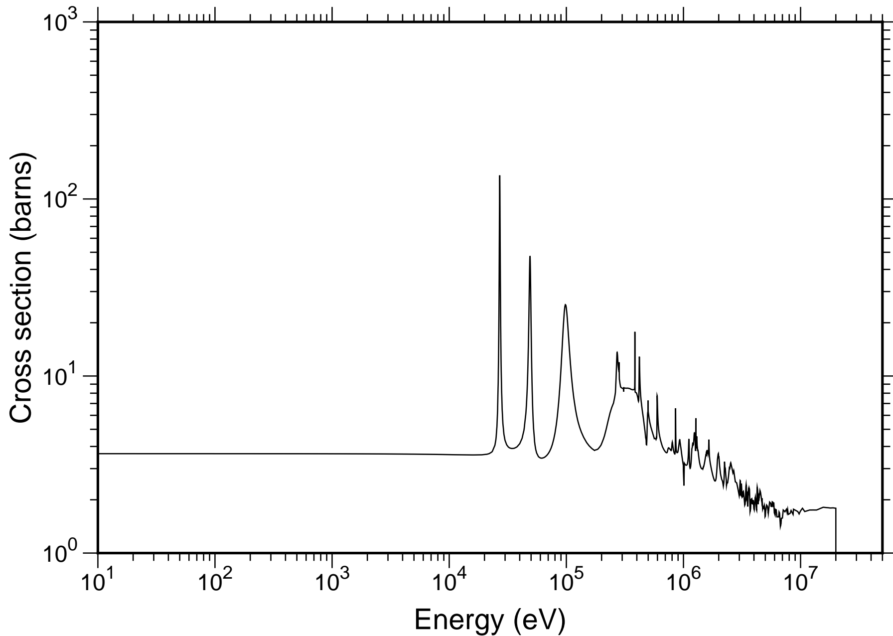
Natural F Total Cross-section - TENDL-2019
