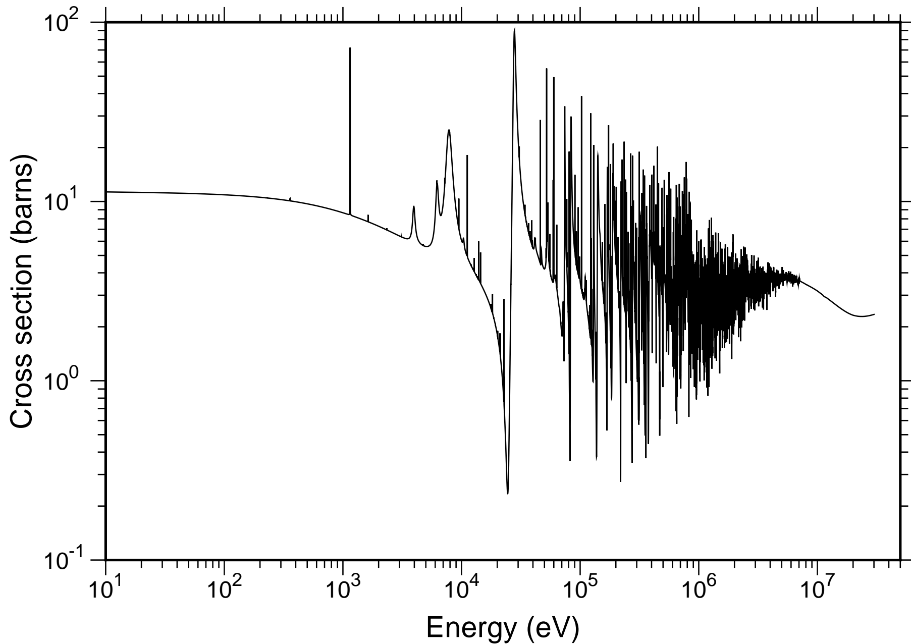
Natural Fe Total Cross-section - TENDL-2019
