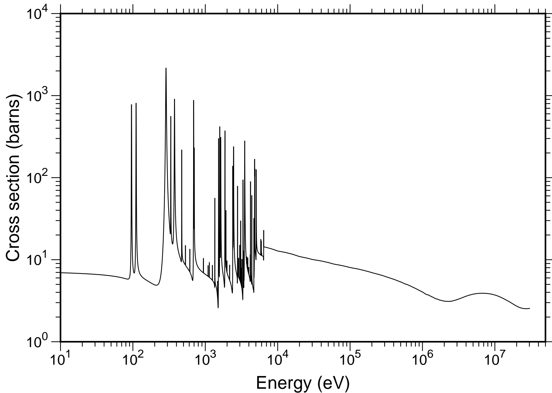
Natural Ga Total Cross-section - TENDL-2019
