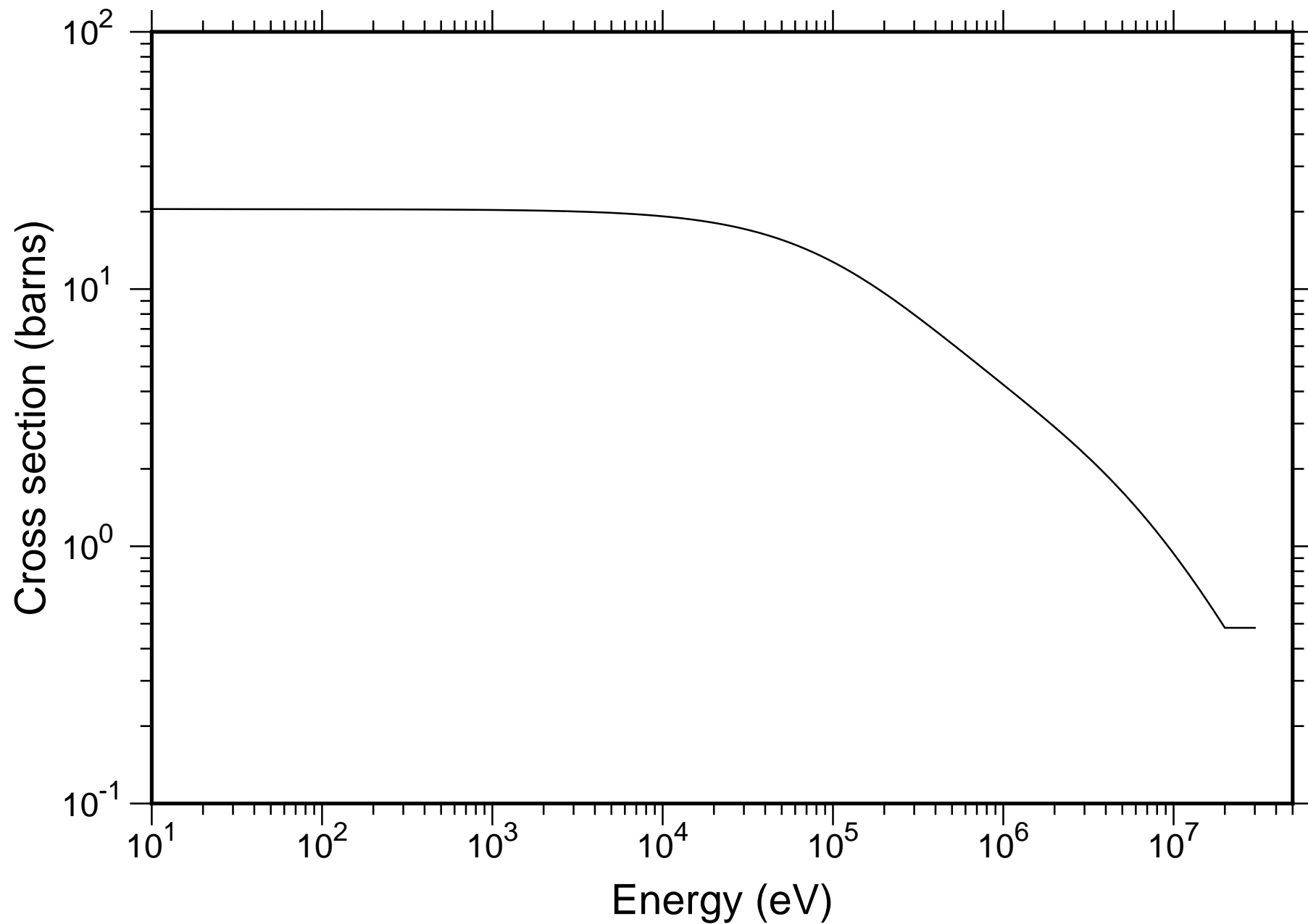
Natural H Total Cross-section - TENDL-2019
