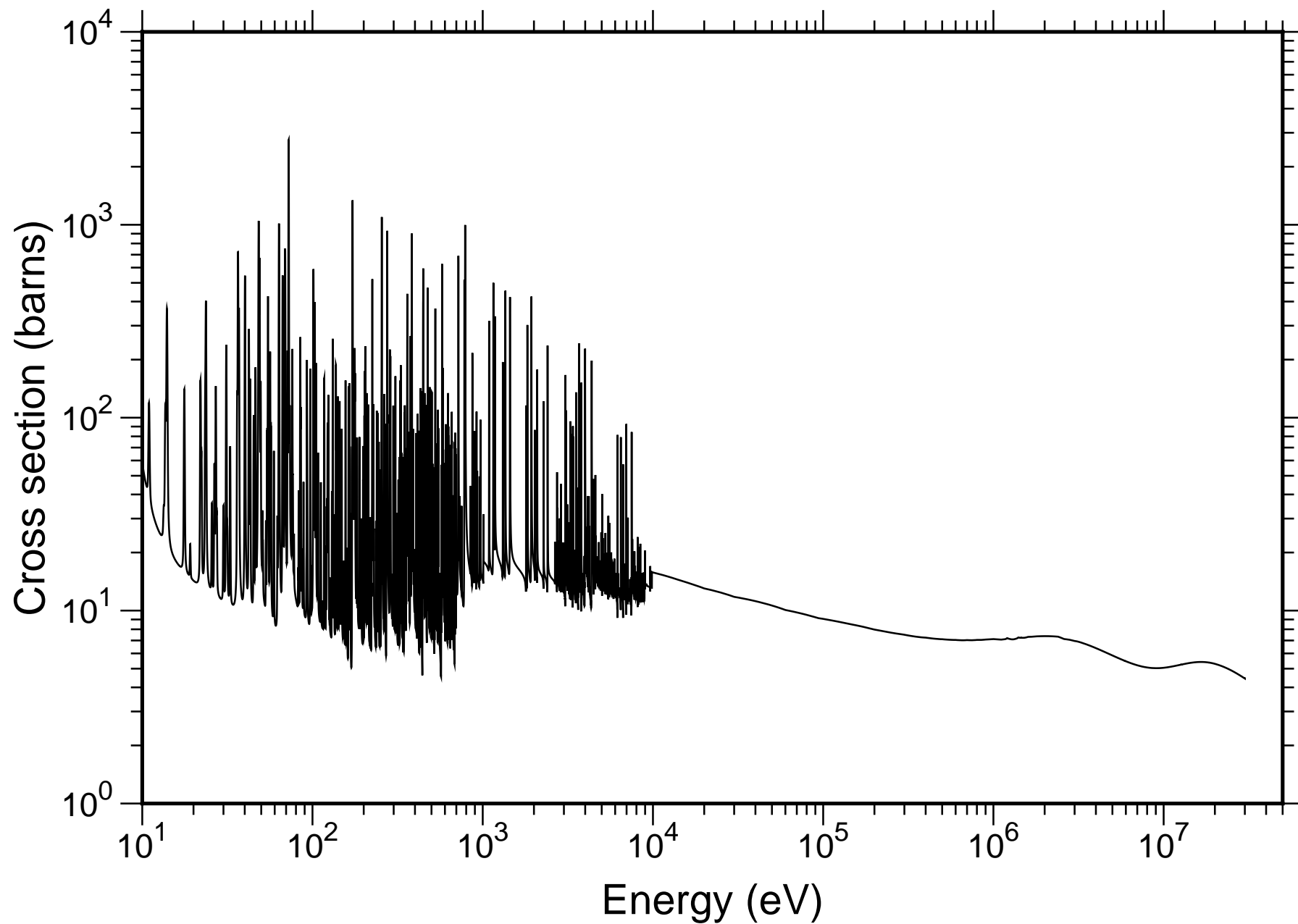
Natural Hf Total Cross-section - TENDL-2019
