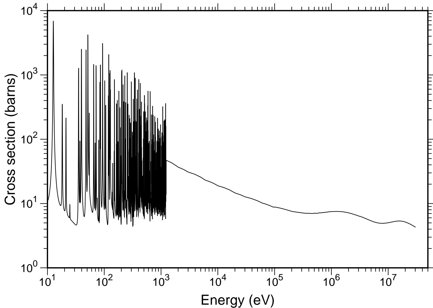
Natural Ho Total Cross-section - TENDL-2019
