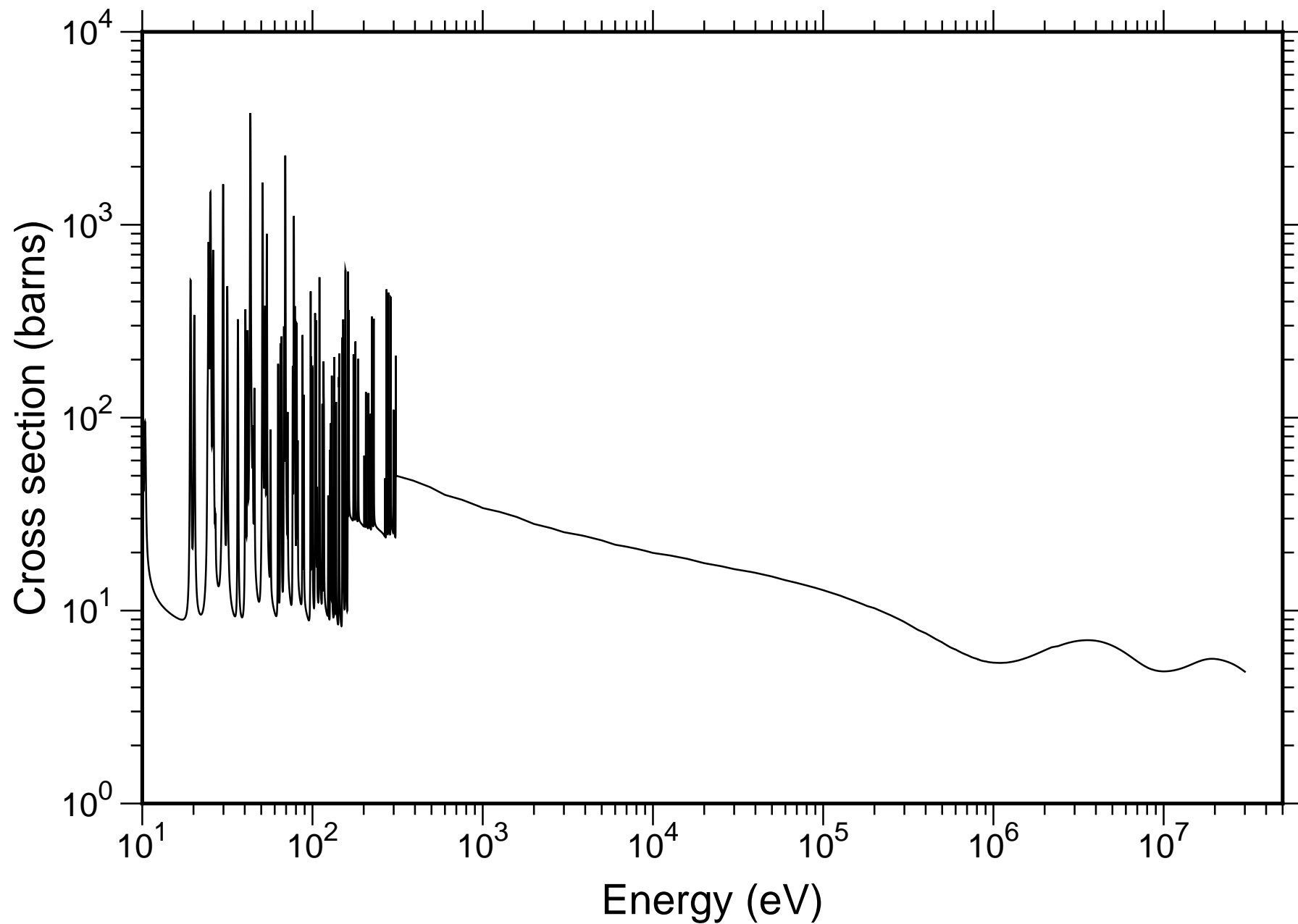
Natural Ir Total Cross-section - TENDL-2019
