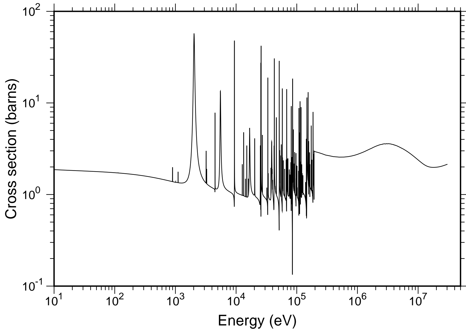
Natural K Total Cross-section - TENDL-2019
