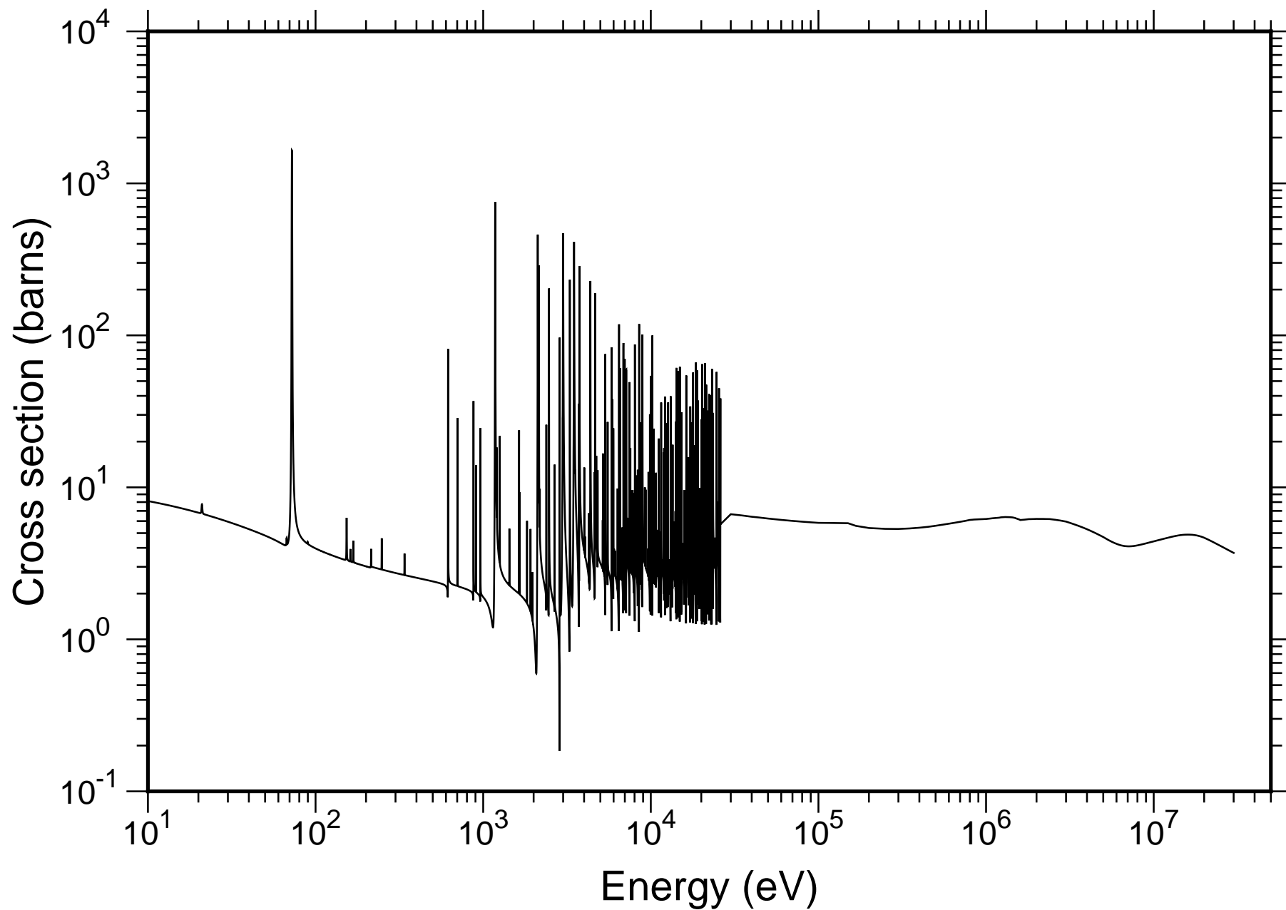
Natural La Total Cross-section - TENDL-2019
