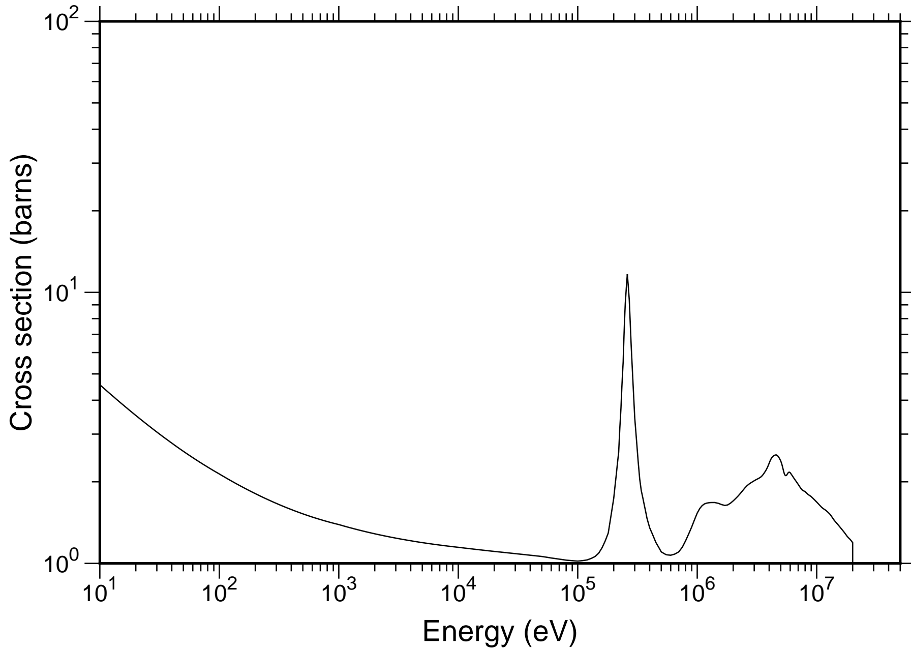
Natural Li Total Cross-section - TENDL-2019
