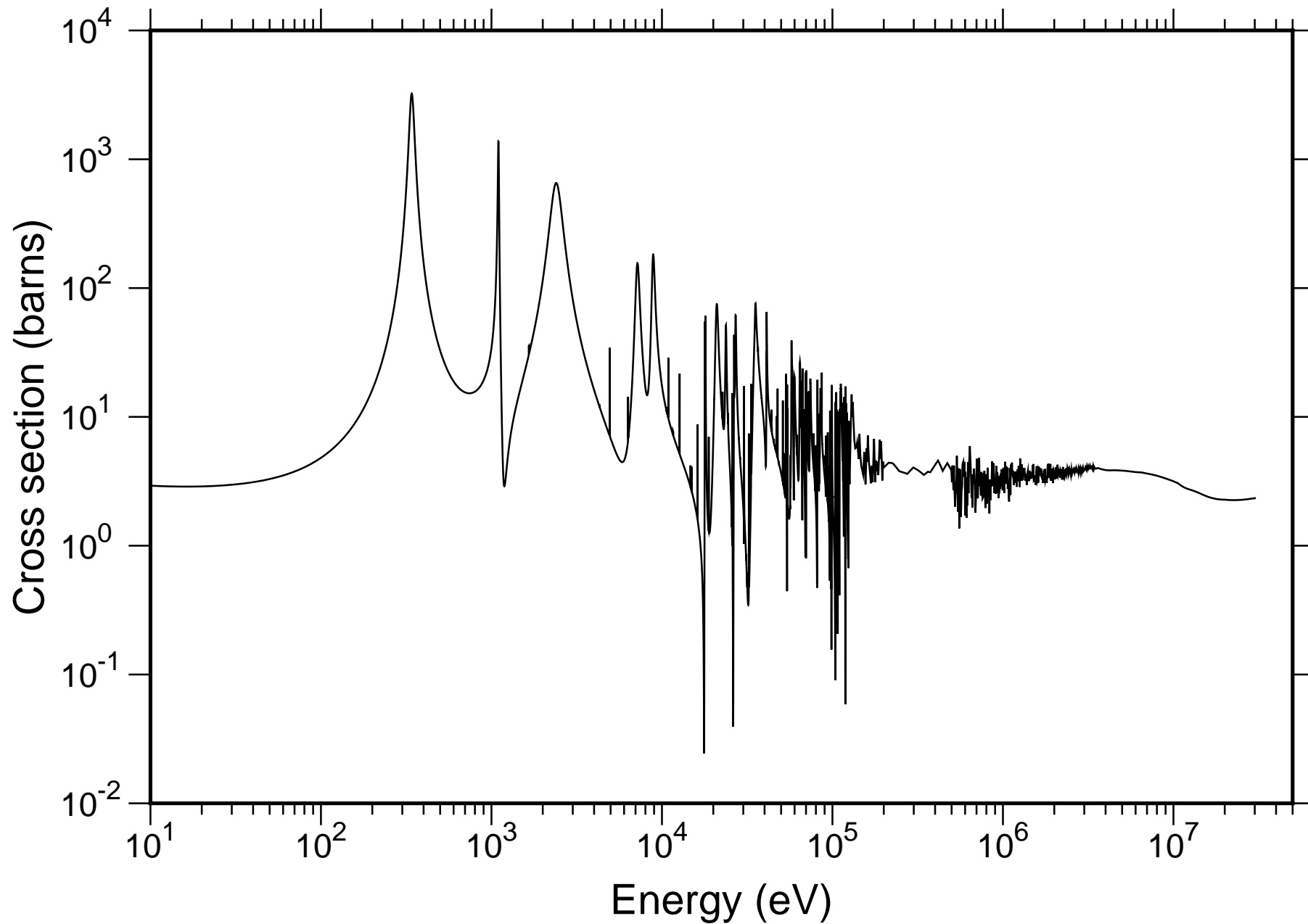
Natural Mn Total Cross-section - TENDL-2019
