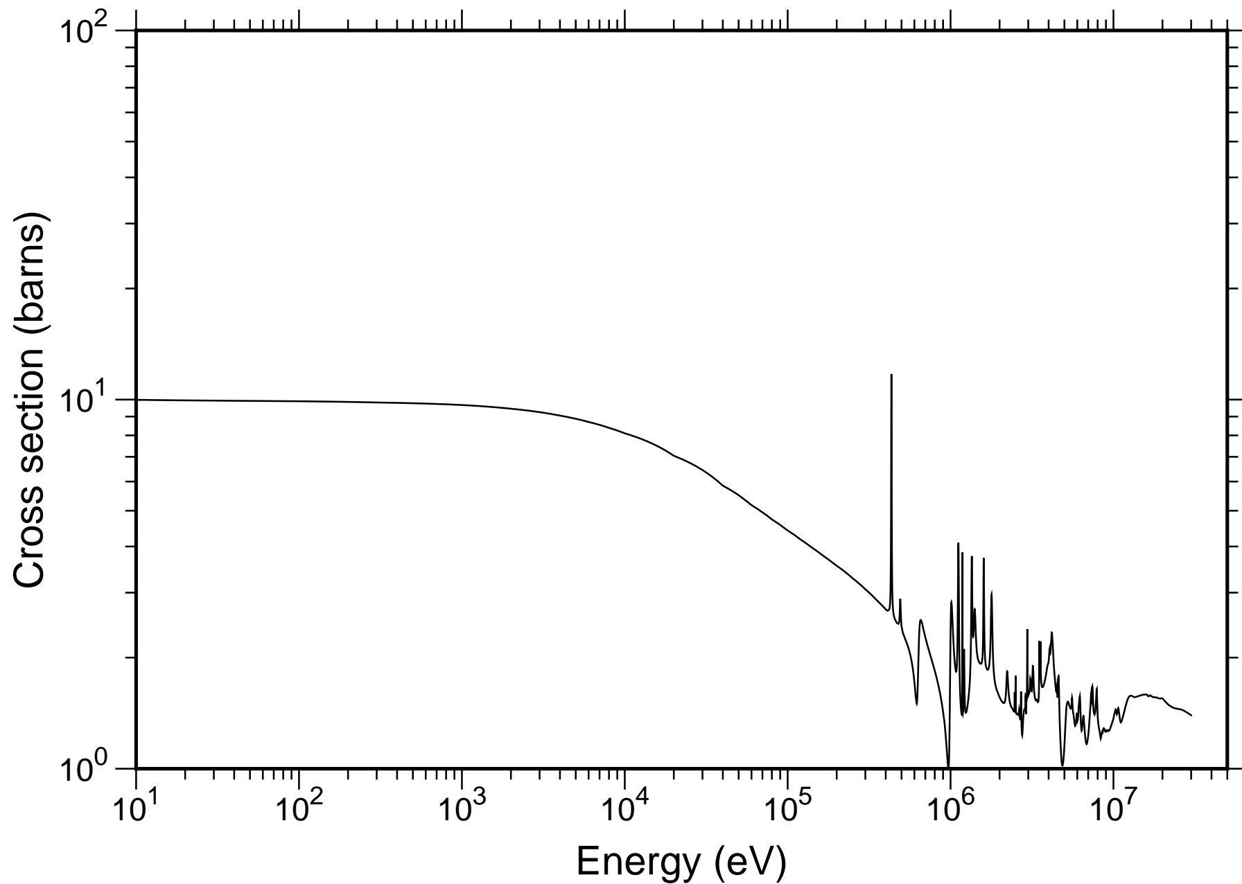
Natural N Total Cross-section - TENDL-2019
