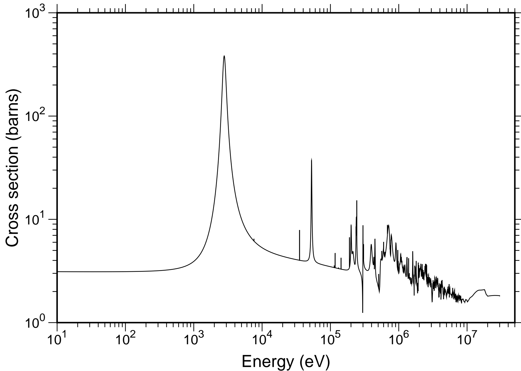
Natural Na Total Cross-section - TENDL-2019
