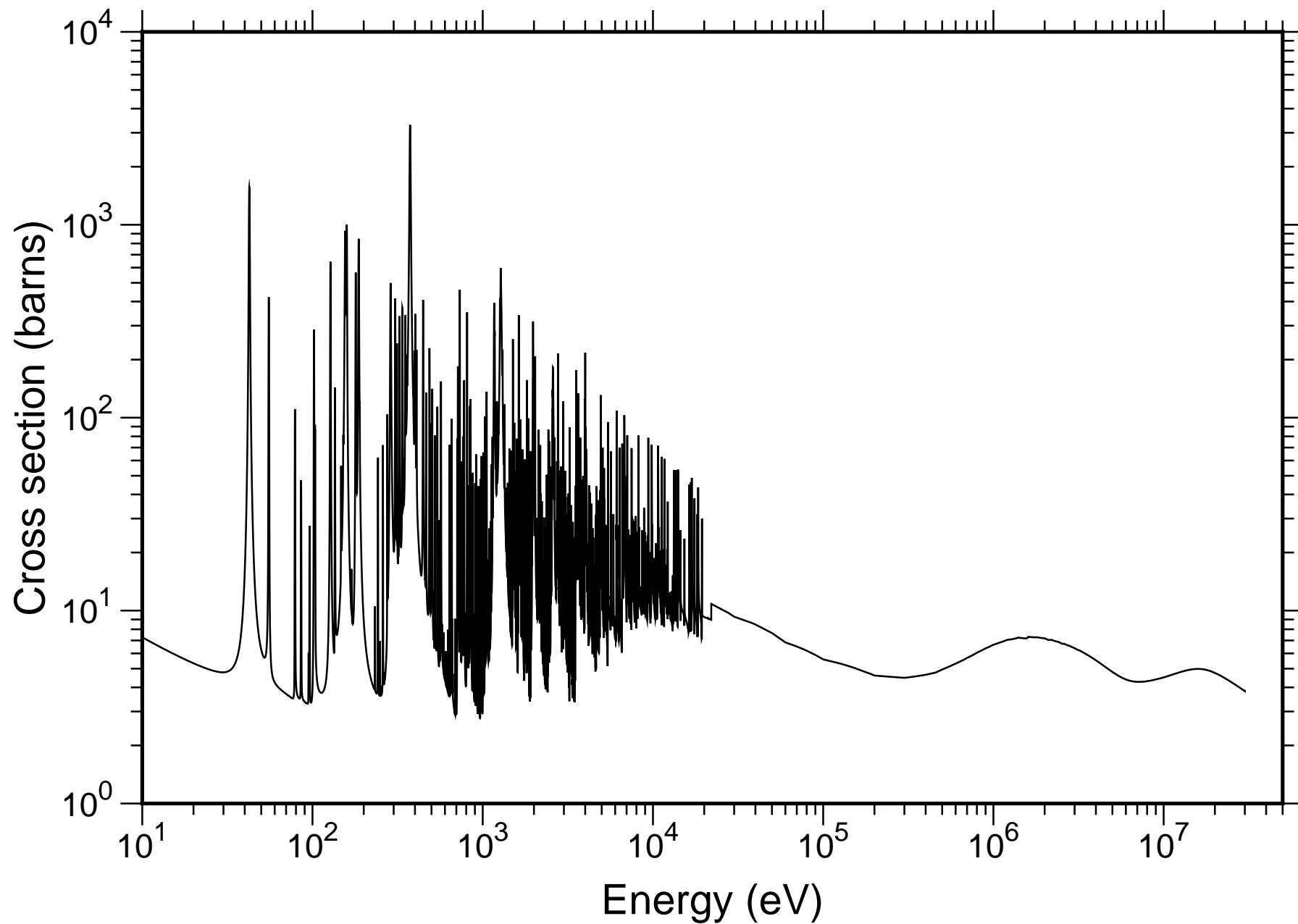
Natural Nd Total Cross-section - TENDL-2019
