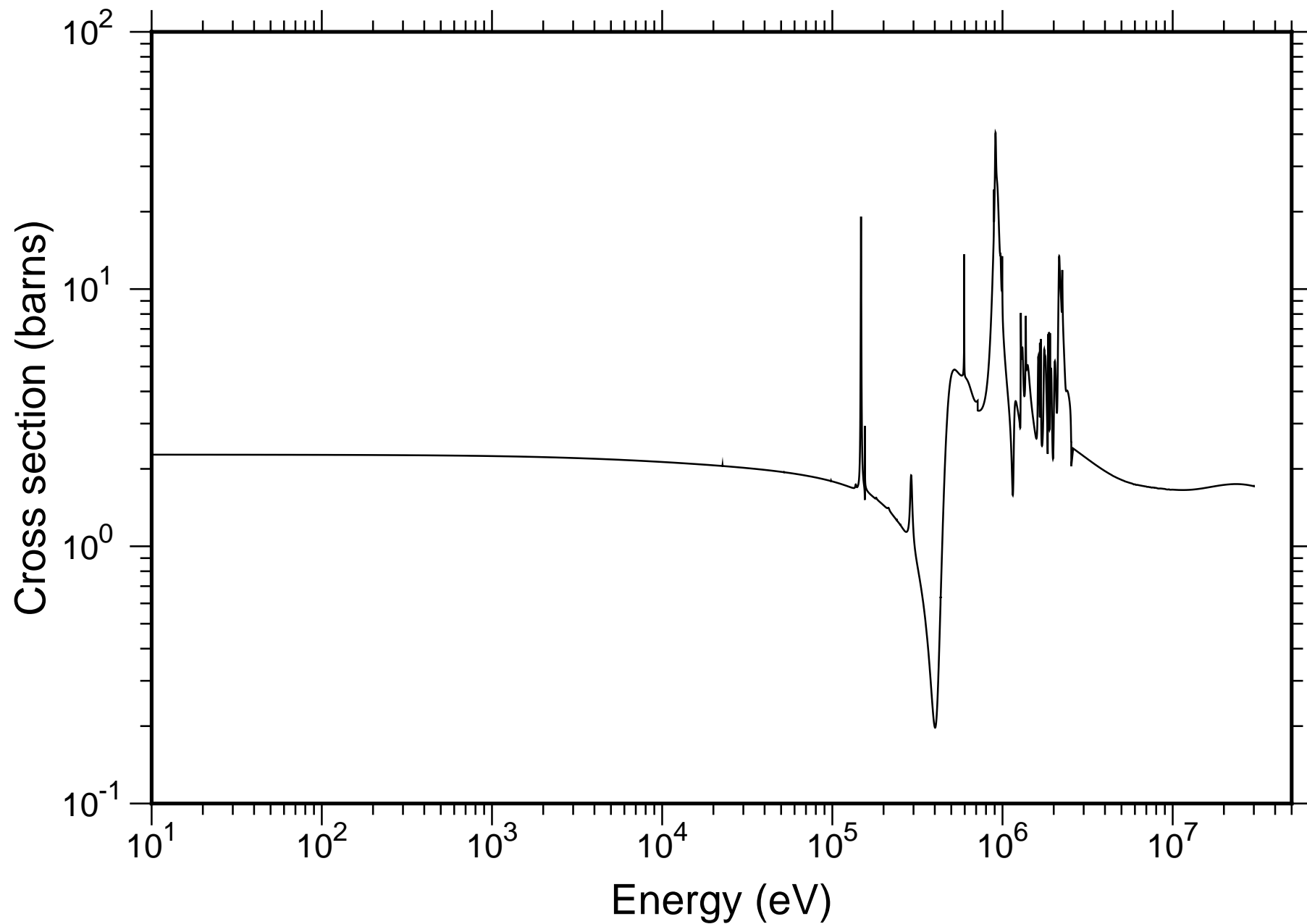
Natural Ne Total Cross-section - TENDL-2019
