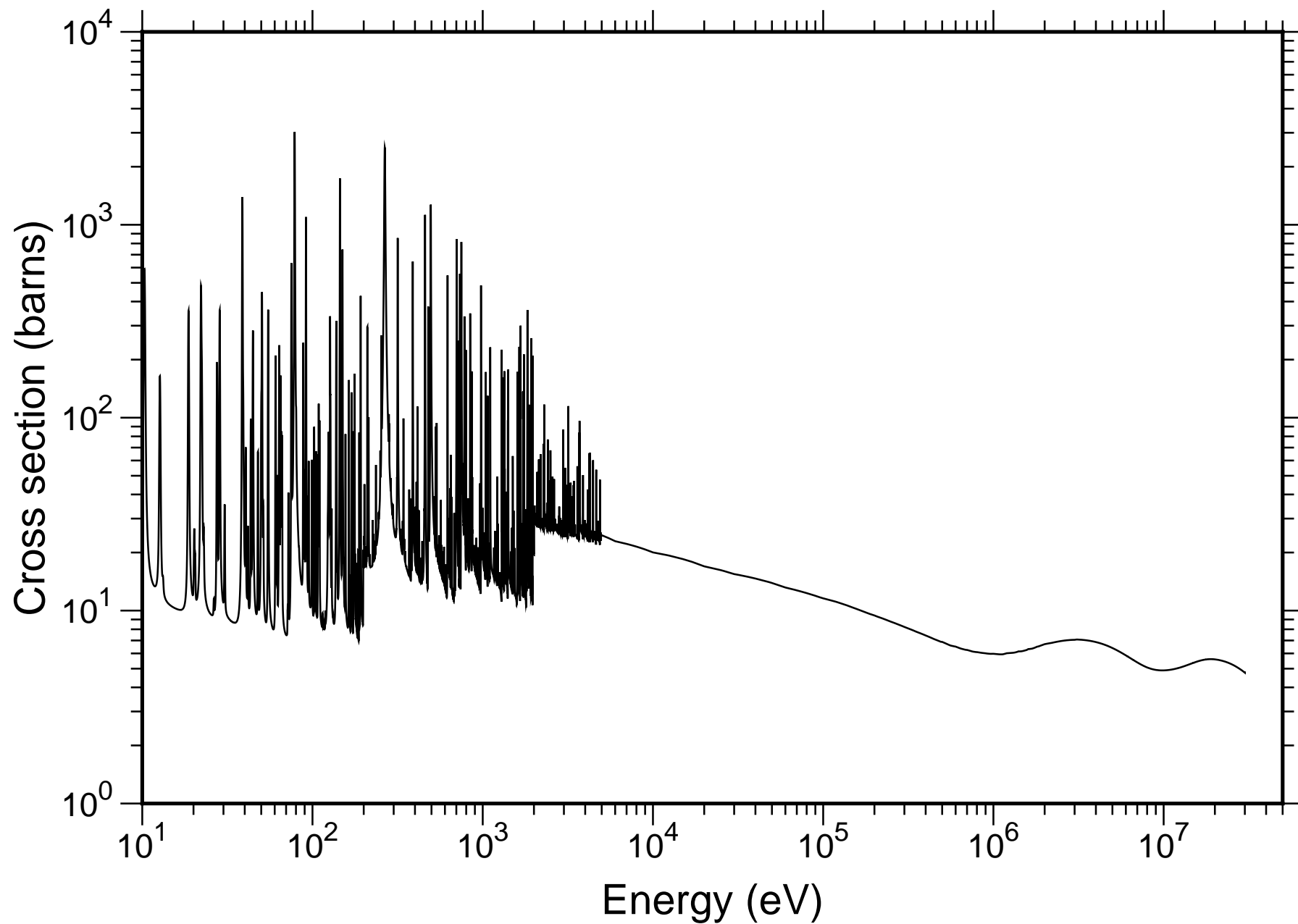
Natural Os Total Cross-section - TENDL-2019
