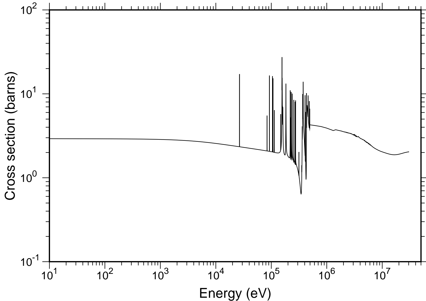
Natural P Total Cross-section - TENDL-2019
