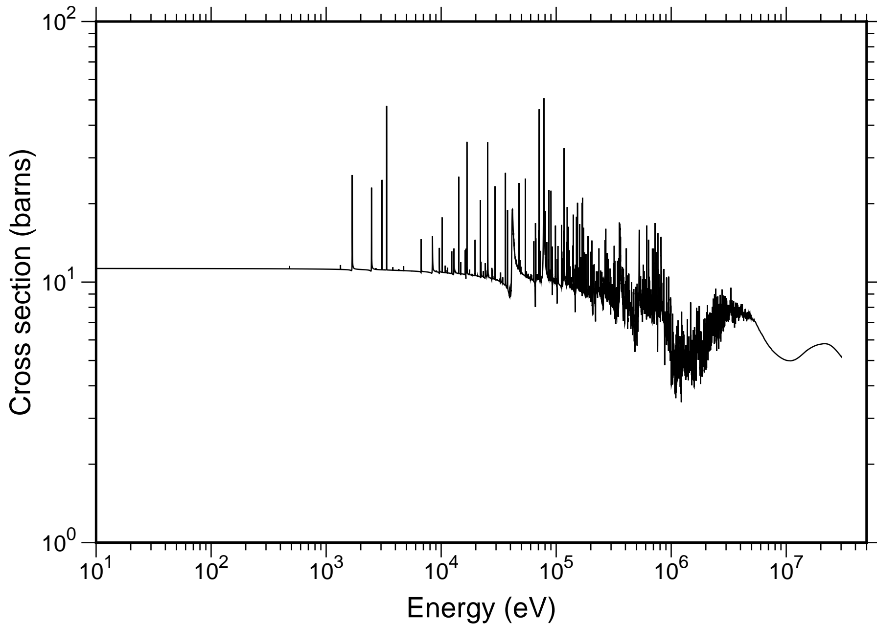
Natural Pb Total Cross-section - TENDL-2019
