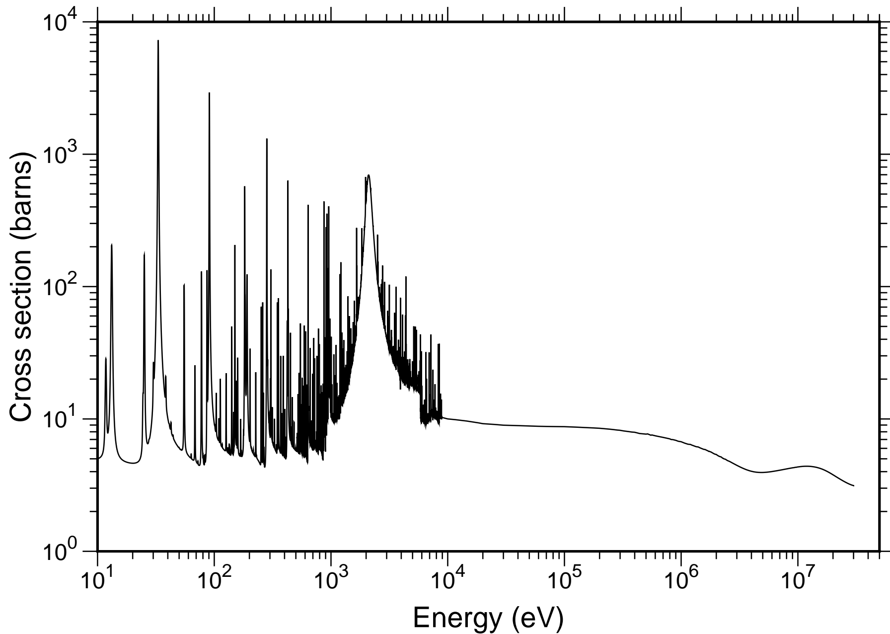
Natural Pd Total Cross-section - TENDL-2019
