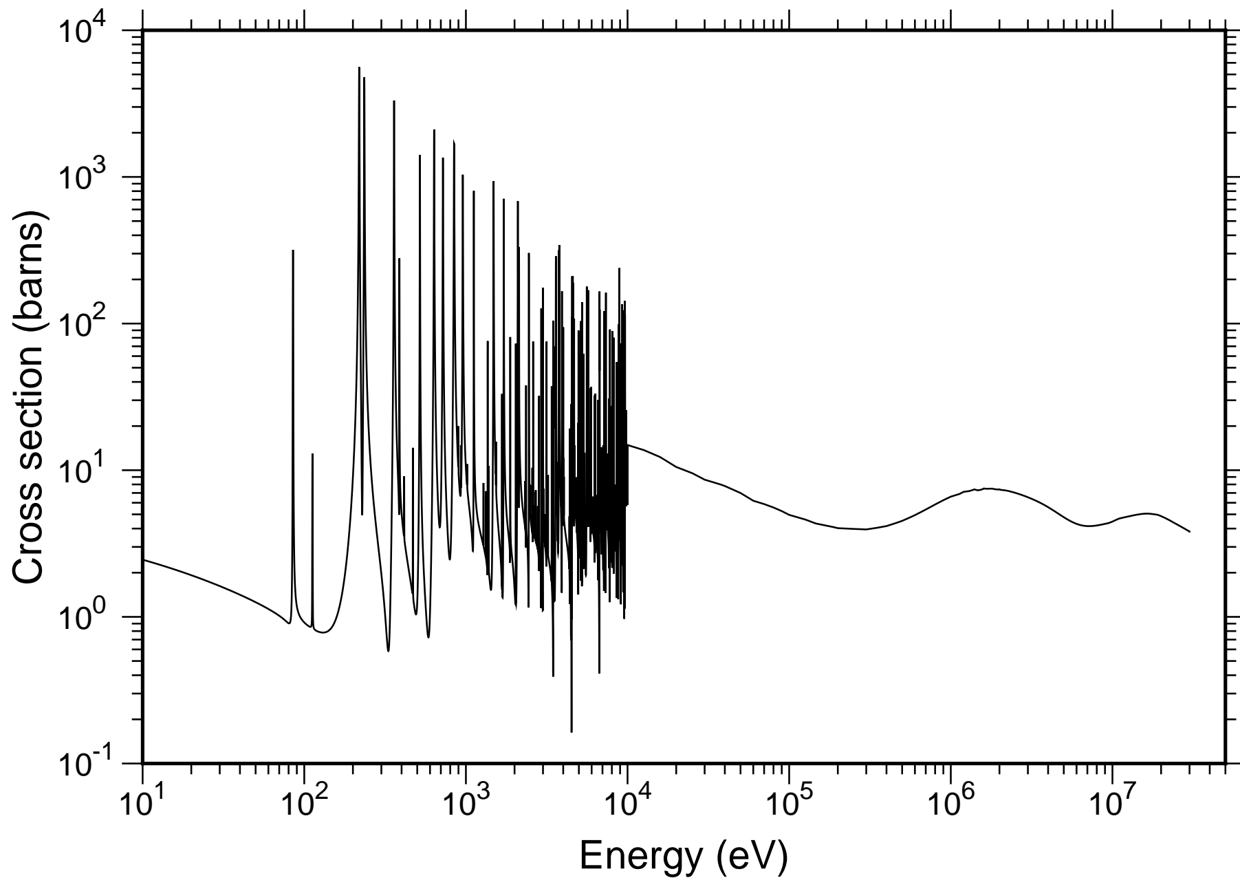
Natural Pr Total Cross-section - TENDL-2019
