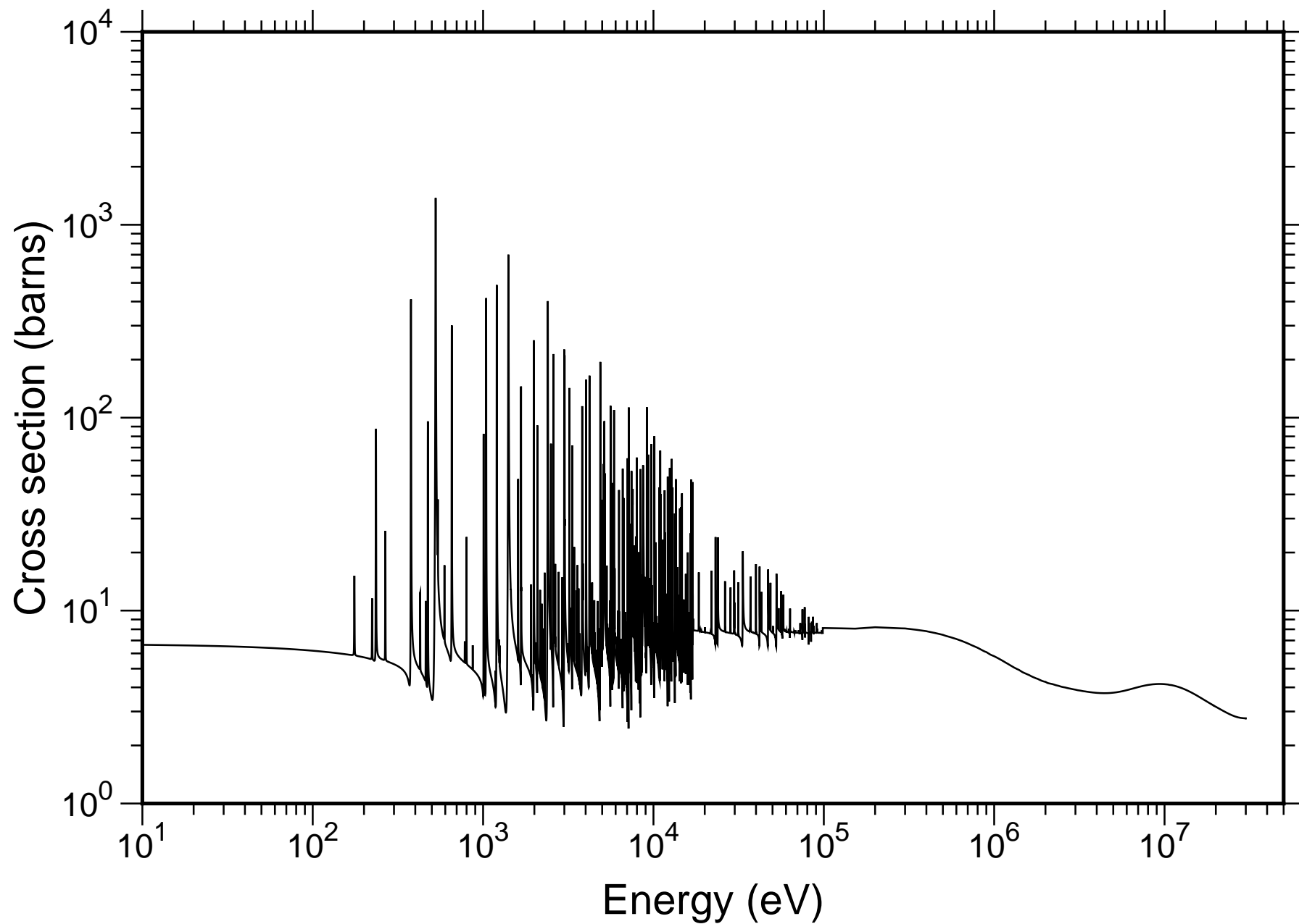
Natural Rb Total Cross-section - TENDL-2019
