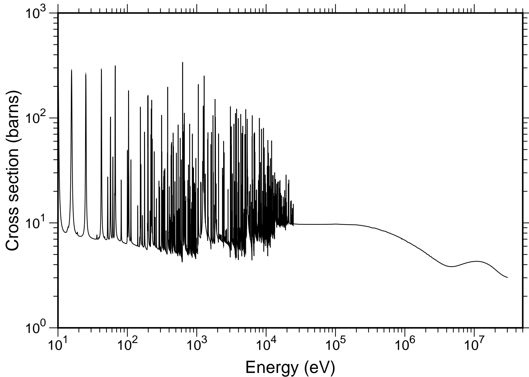
Natural Ru Total Cross-section - TENDL-2019
