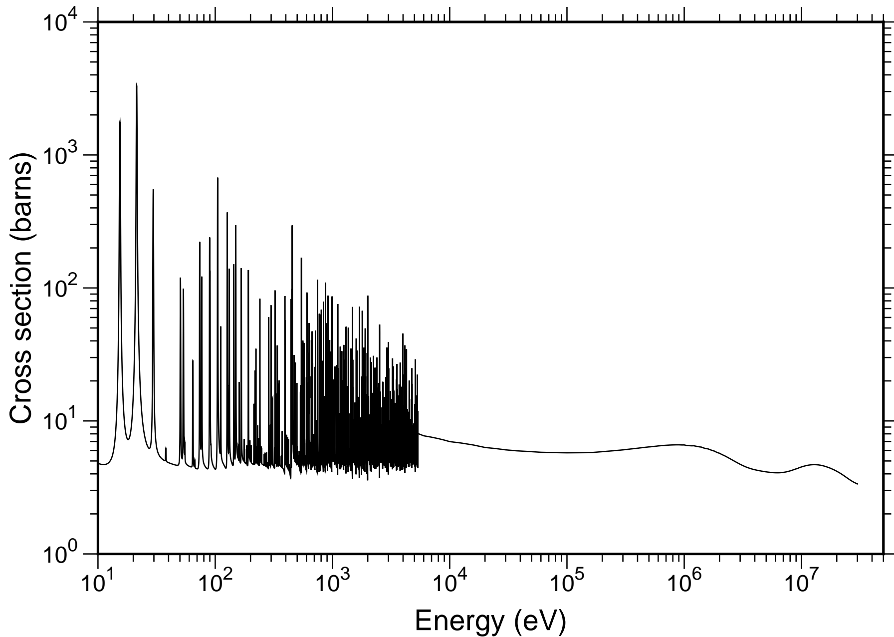
Natural Sb Total Cross-section - TENDL-2019
