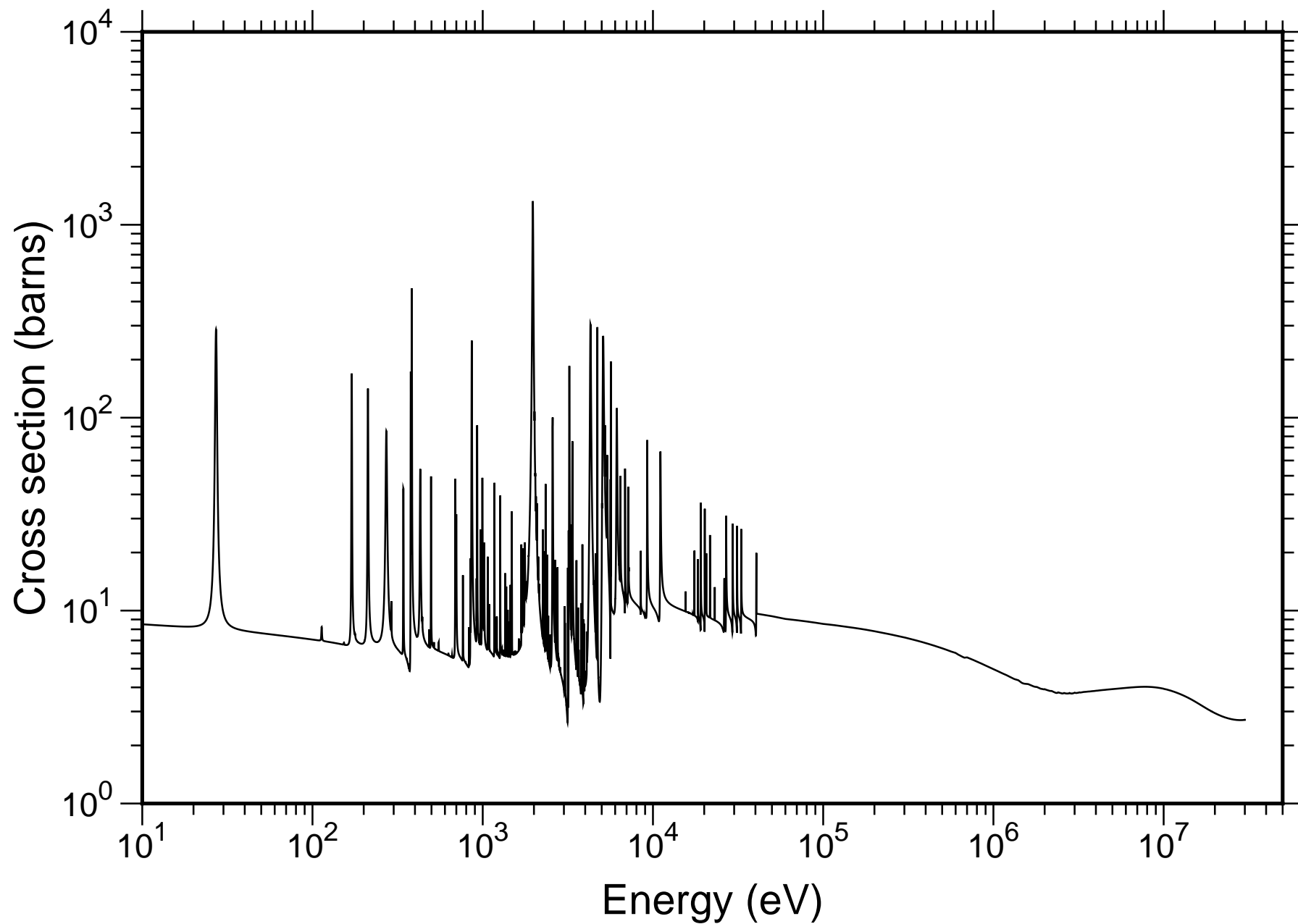
Natural Se Total Cross-section - TENDL-2019
