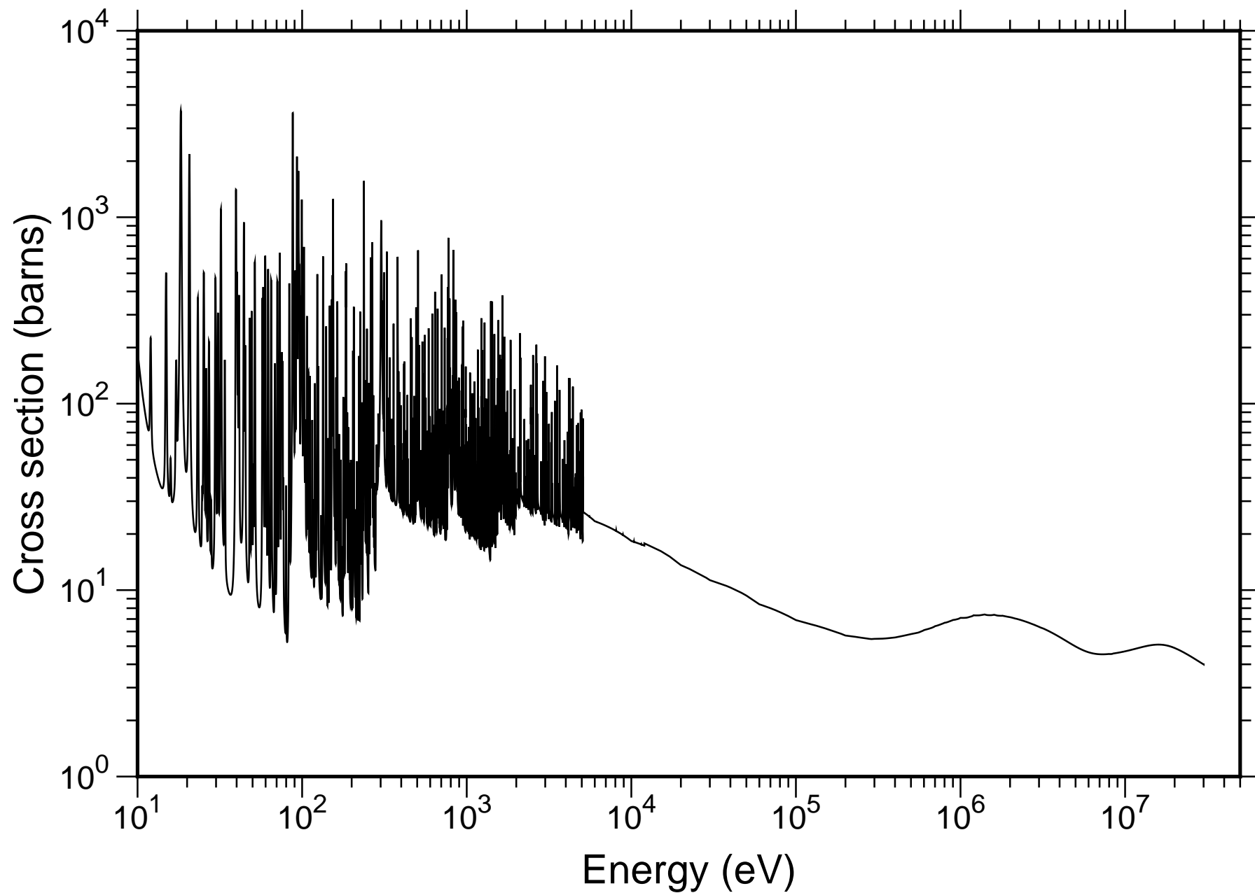
Natural Sm Total Cross-section - TENDL-2019
