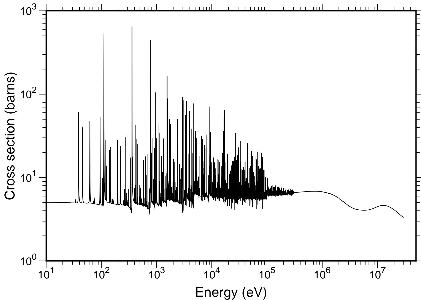
Natural Sn Total Cross-section - TENDL-2019
