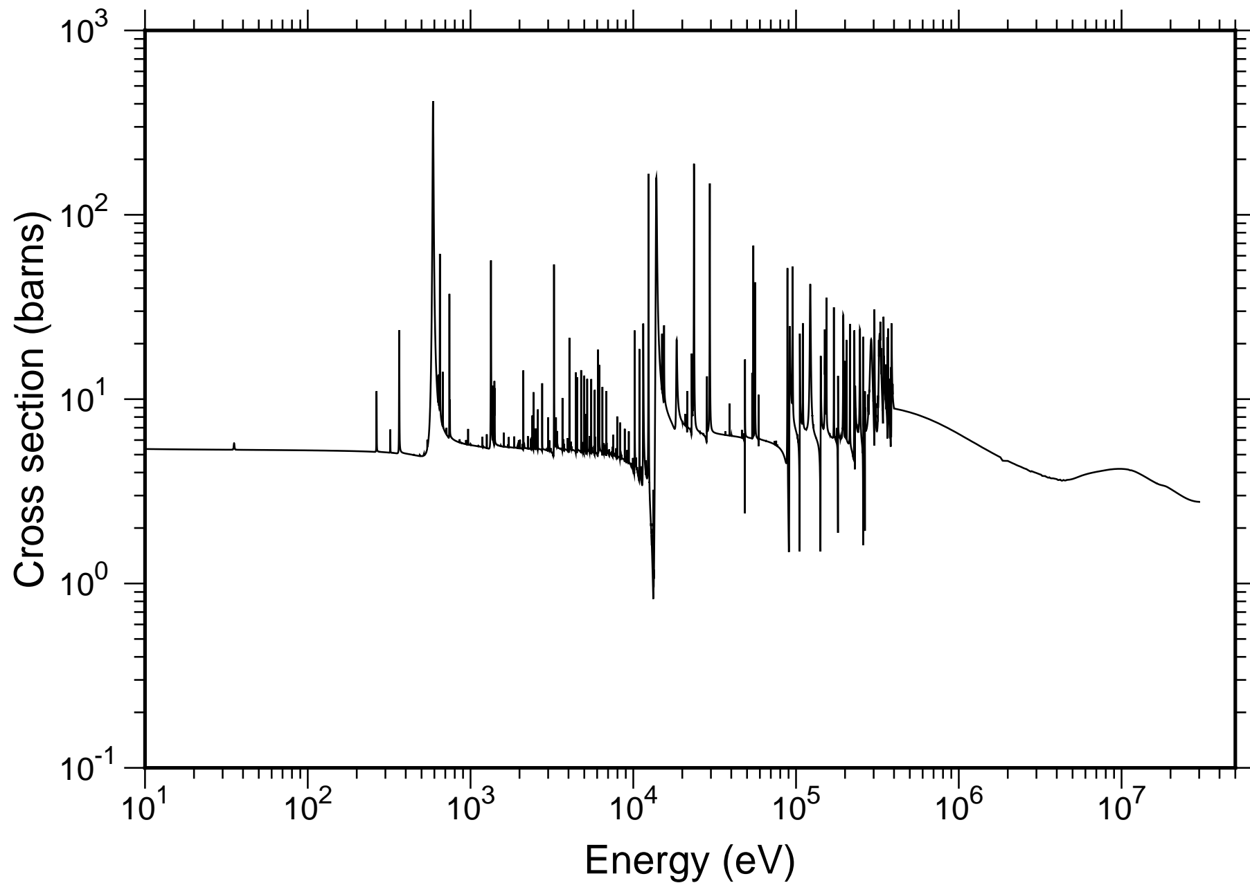
Natural Sr Total Cross-section - TENDL-2019
