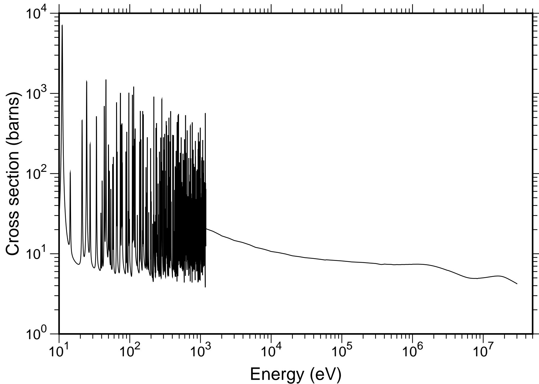
Natural Tb Total Cross-section - TENDL-2019
