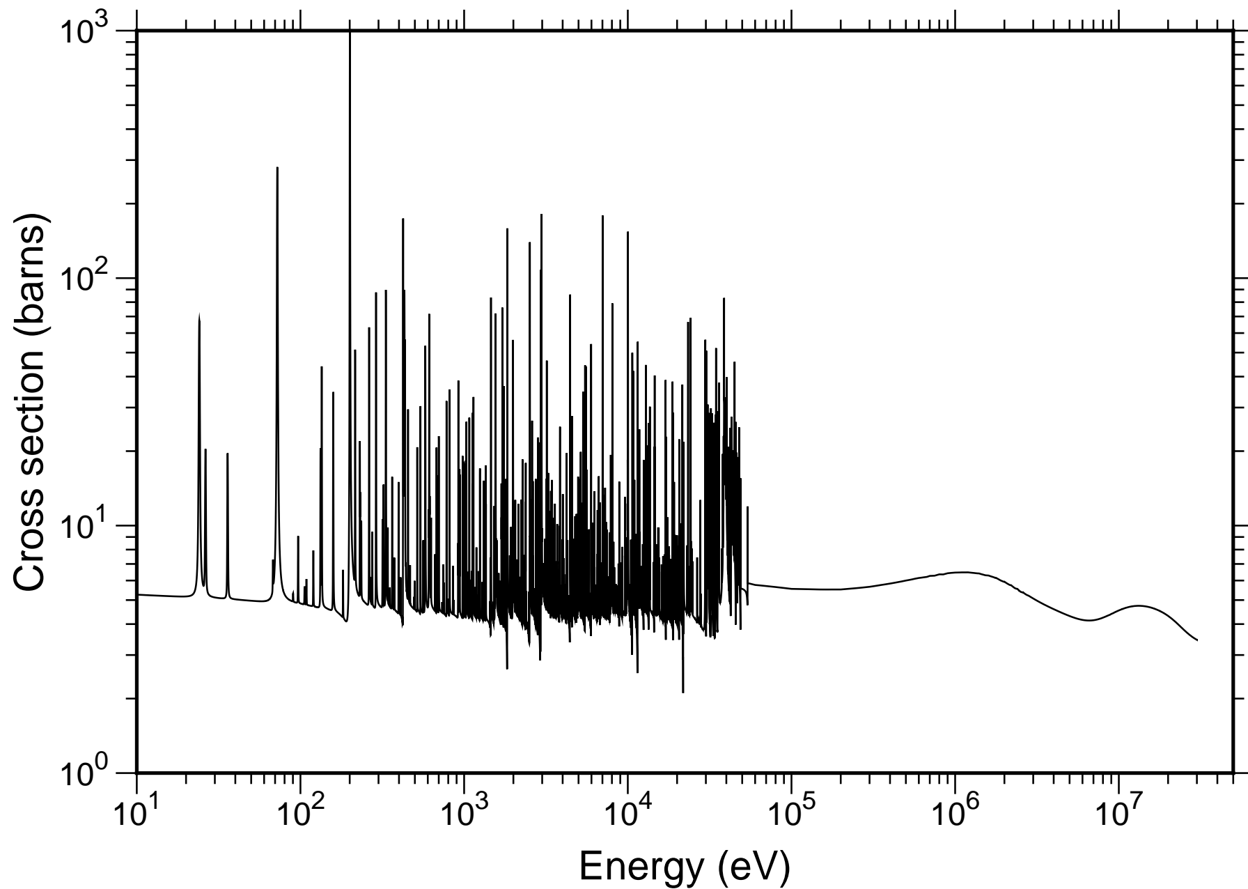
Natural Te Total Cross-section - TENDL-2019
