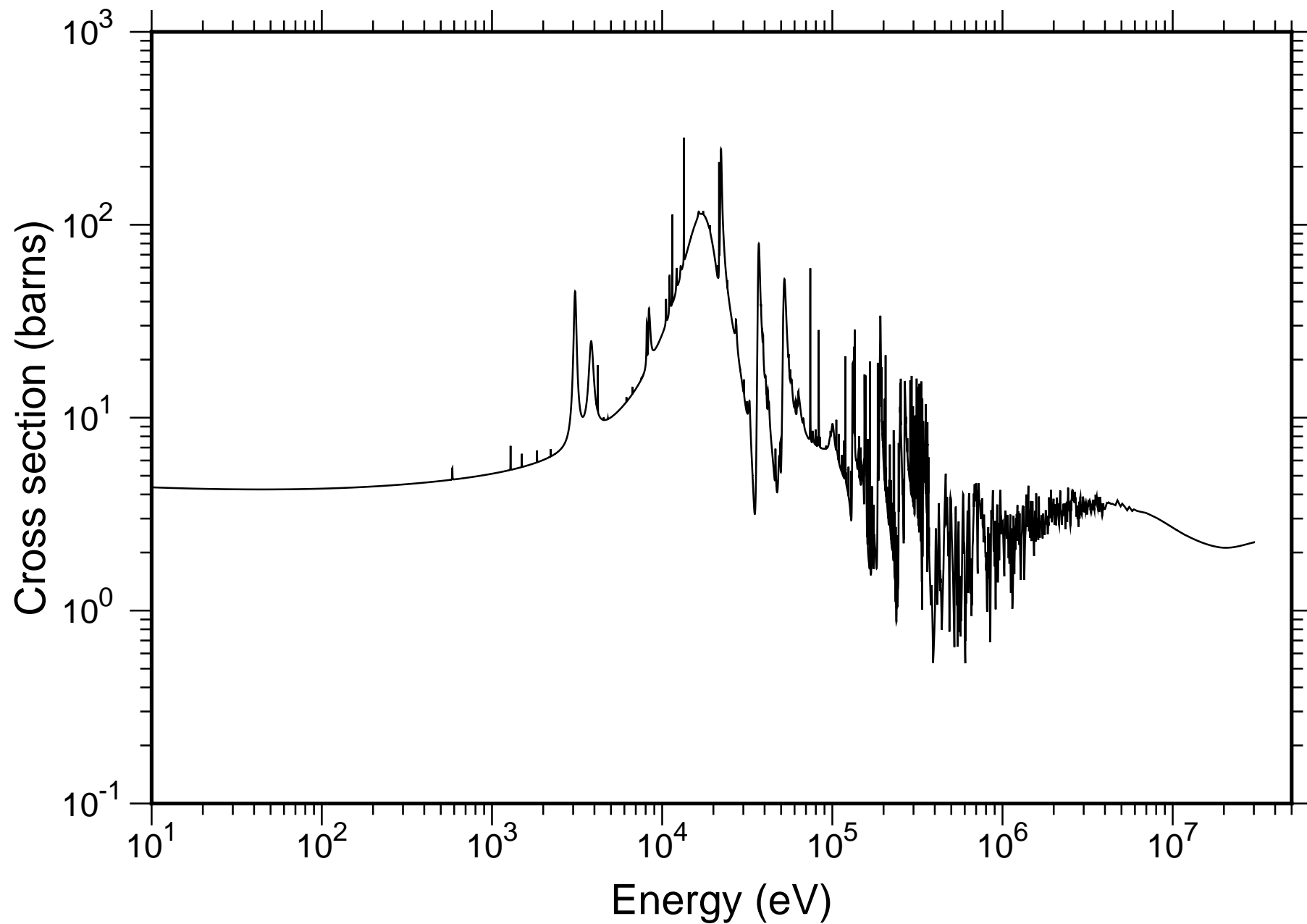
Natural Ti Total Cross-section - TENDL-2019
