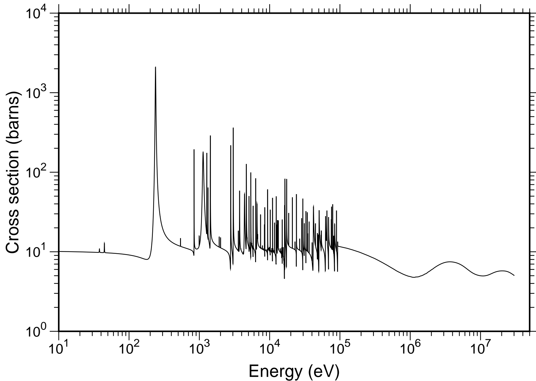
Natural TI Total Cross-section - TENDL-2019
