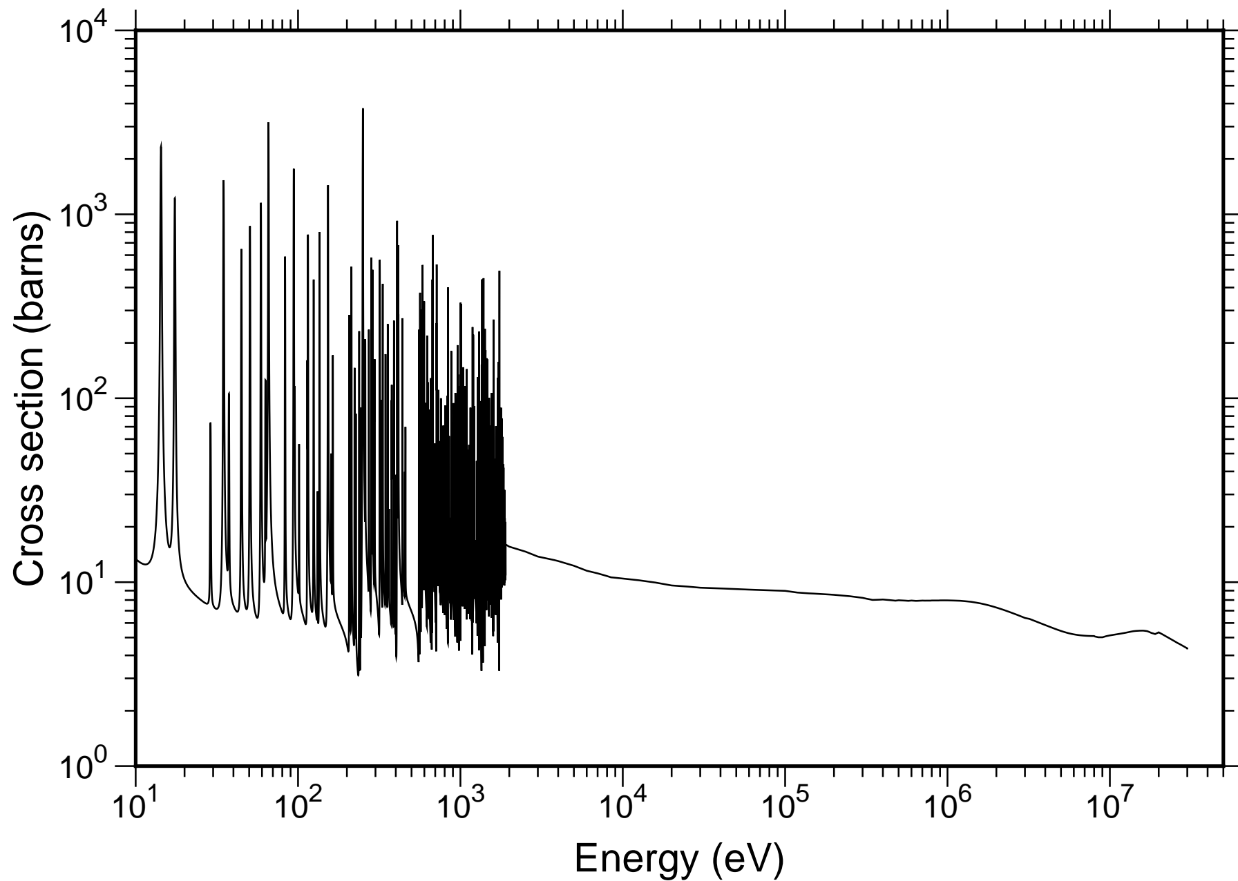
Natural Tm Total Cross-section - TENDL-2019
