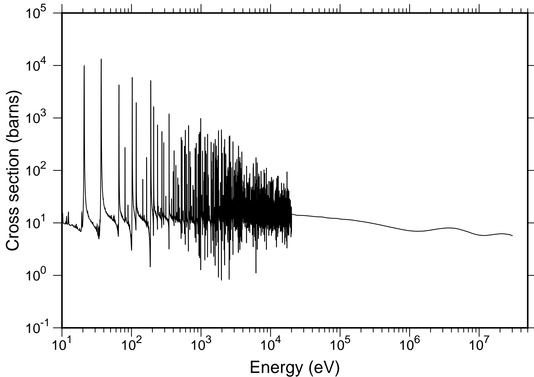
Natural U Total Cross-section - TENDL-2019
