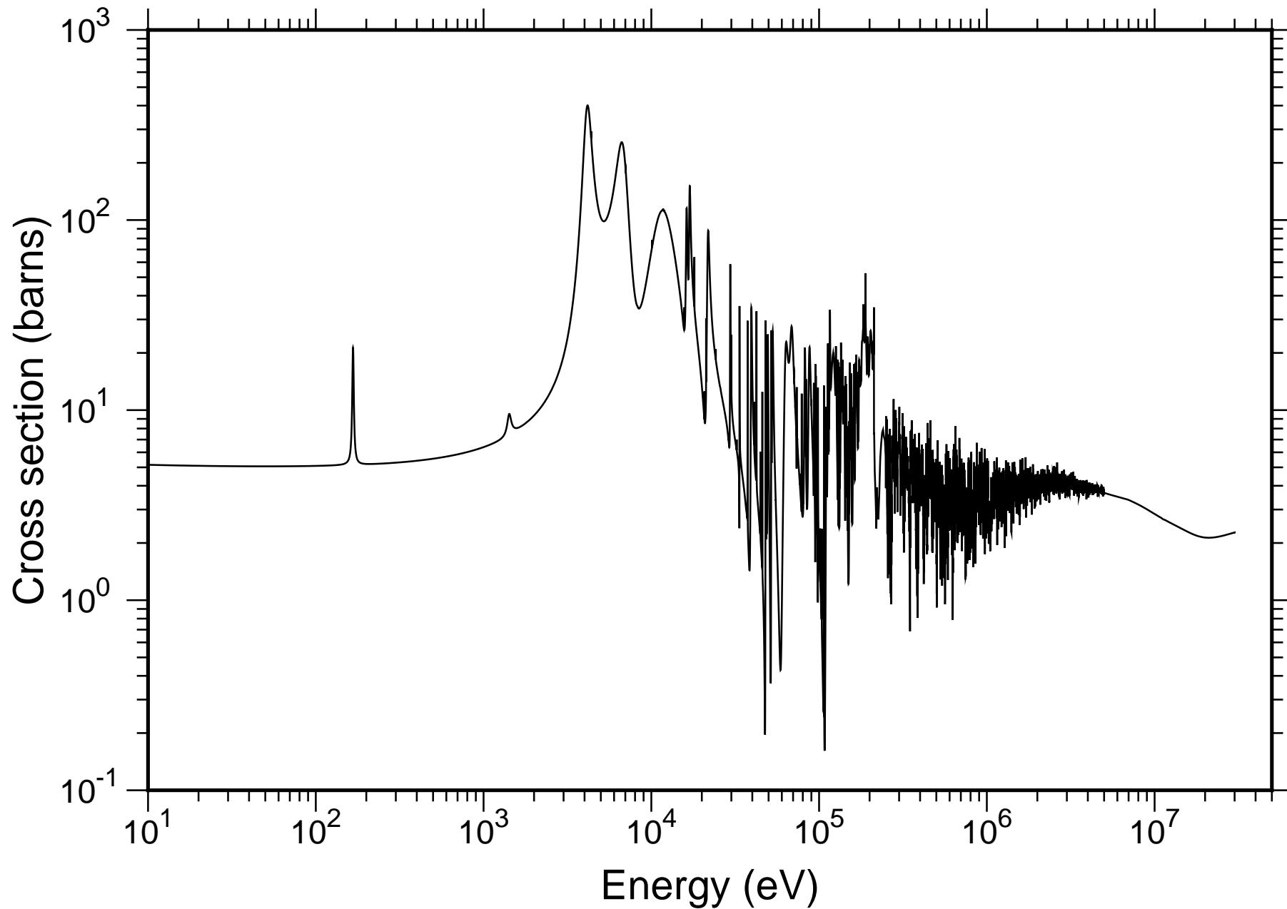
Natural V Total Cross-section - TENDL-2019
