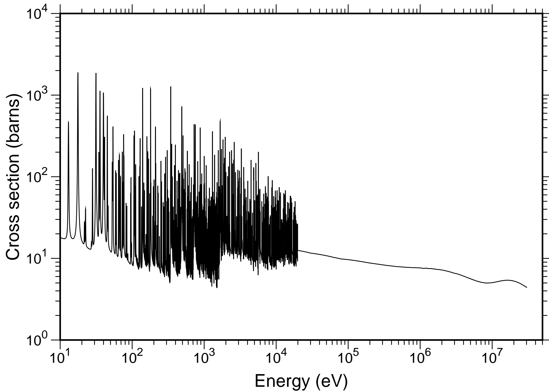
Natural Yb Total Cross-section - TENDL-2019
