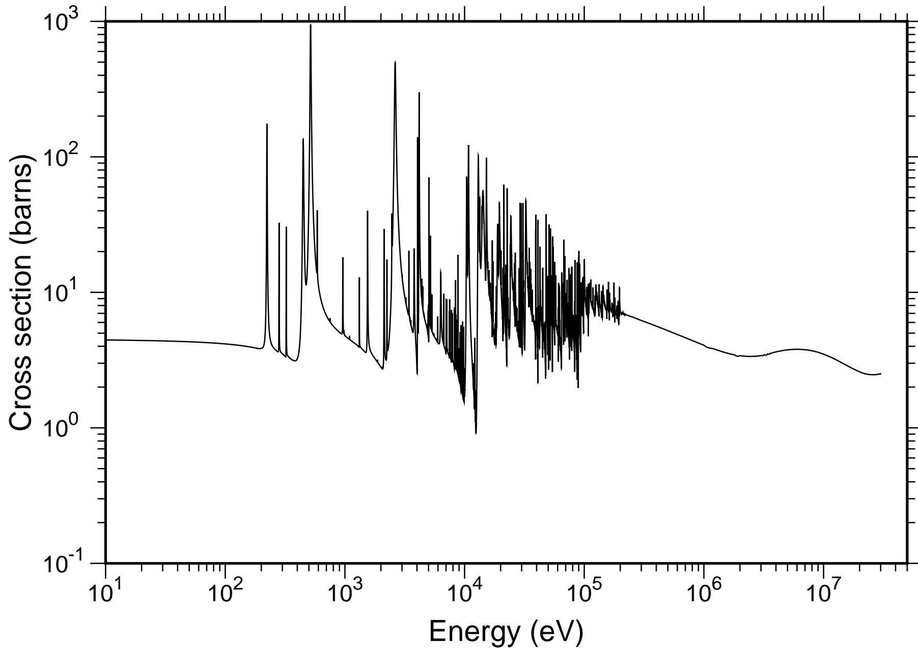
Natural Zn Total Cross-section - TENDL-2019
