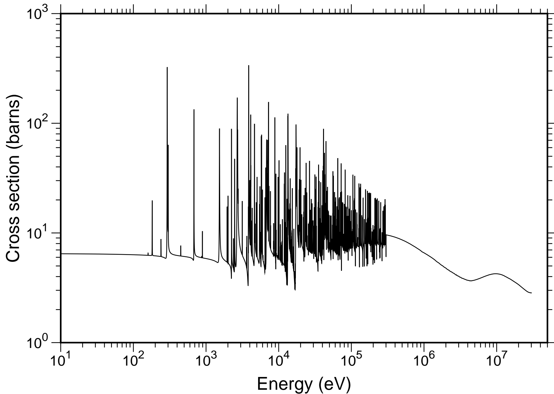
Natural Zr Total Cross-section - TENDL-2019
