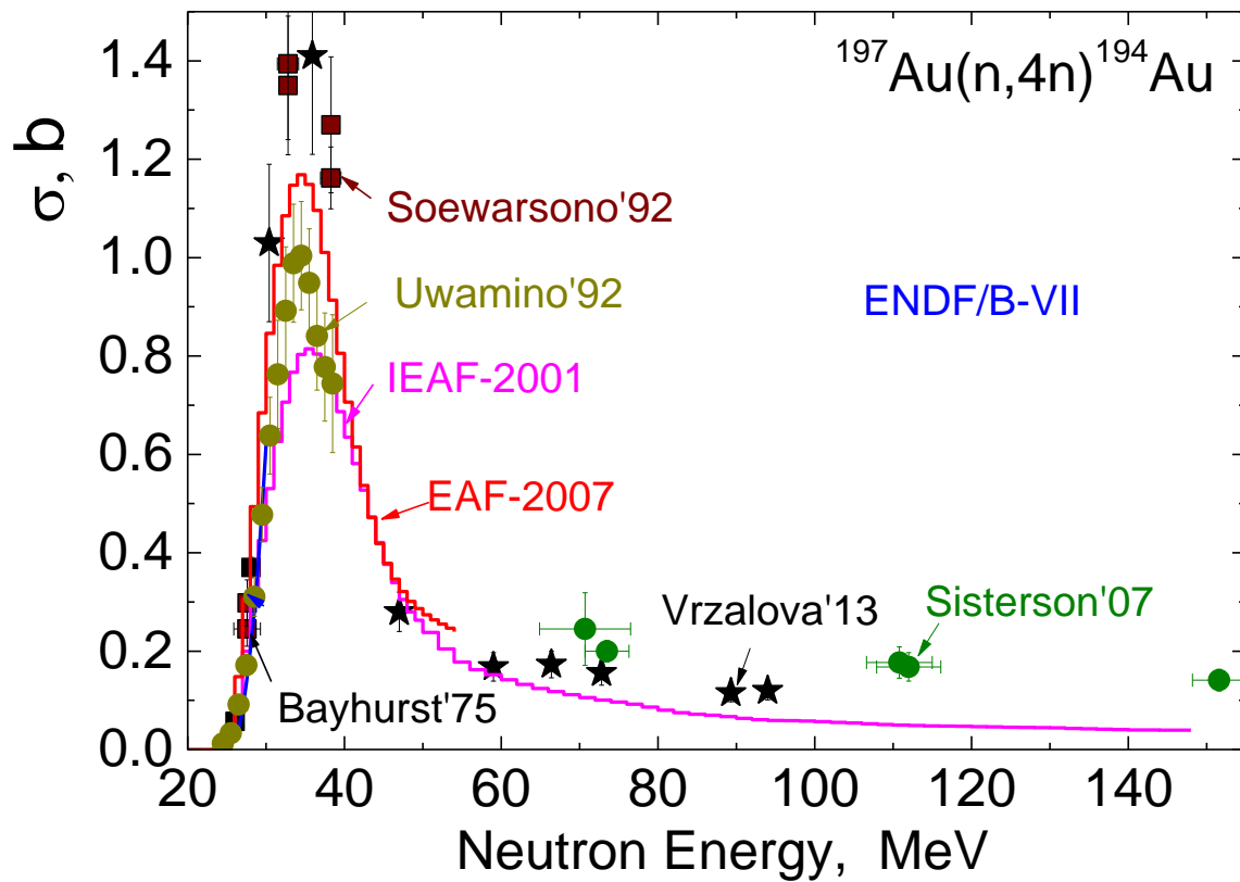
Fig. 2. The ^{197}\text{Au}(n,4n)^{194}\text{Au} cross sections.
