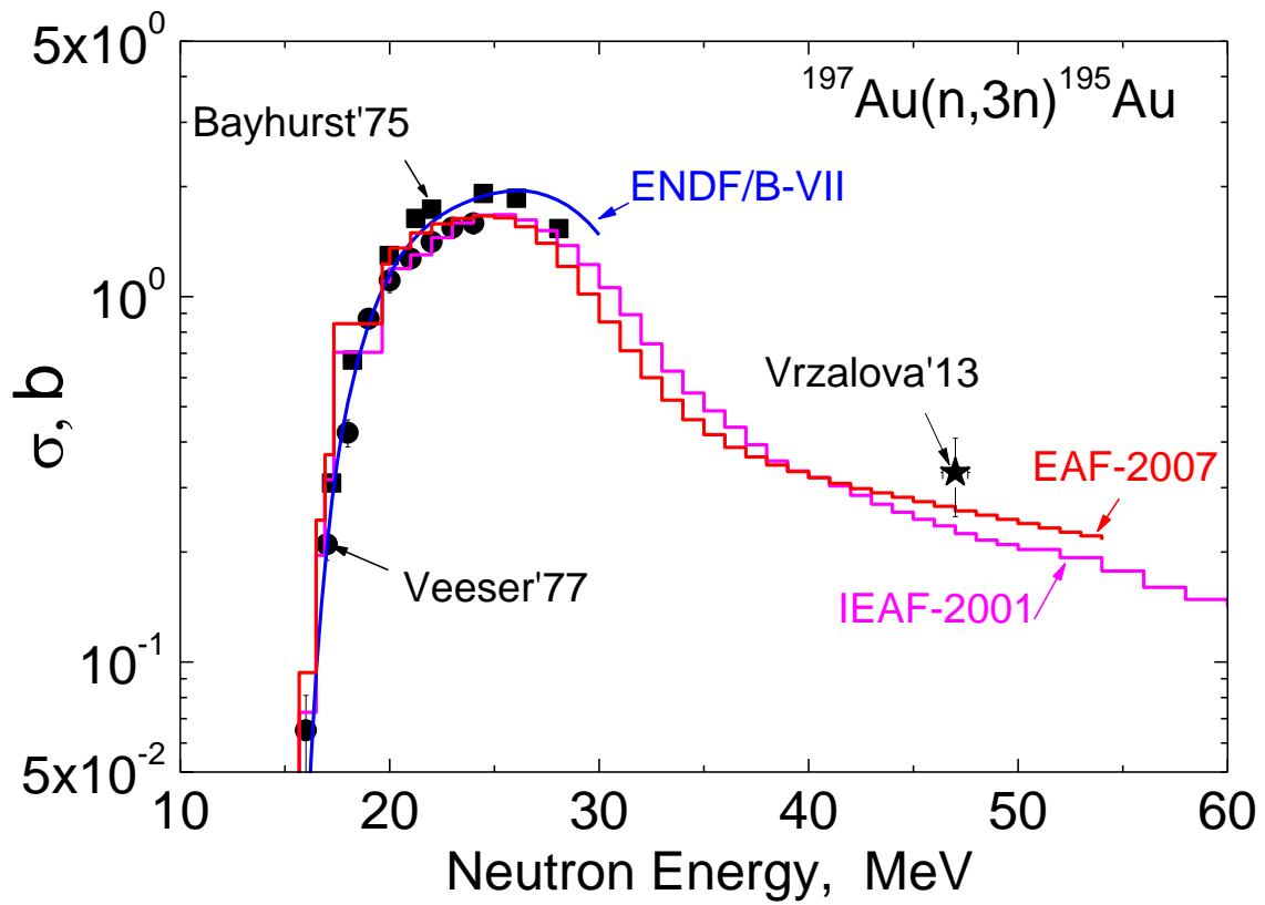
Fig. 1. The ^{197}\text{Au}(n,3n)^{195}\text{Au} cross sections
