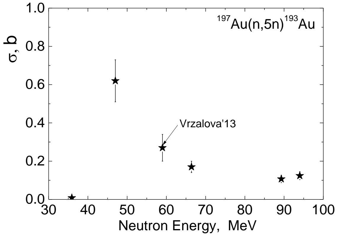
Fig. 3. The ^{197}\text{Au}(n,5n)^{193}\text{Au} cross sections.
