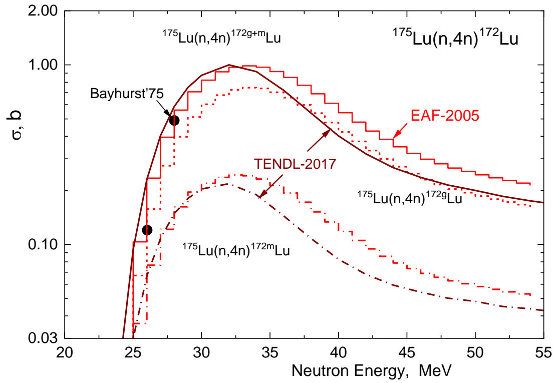
Fig. 3. The ^{175}\text{Lu}(n,4n)^{172}\text{Lu} cross sections.
