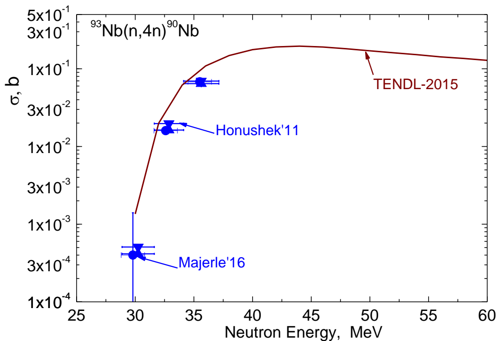
Fig. 2. Cross sections for the ^{93}\text{Nb}(n,4n)^{90}\text{Nb} reaction: experimental data from EXFOR (points) and evaluations (curves).
