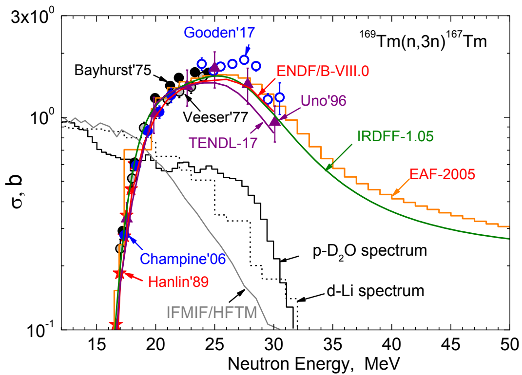
Fig. 2. ^{169}\text{Tm}(n,3n)^{167}\text{Tm} reaction cross sections
