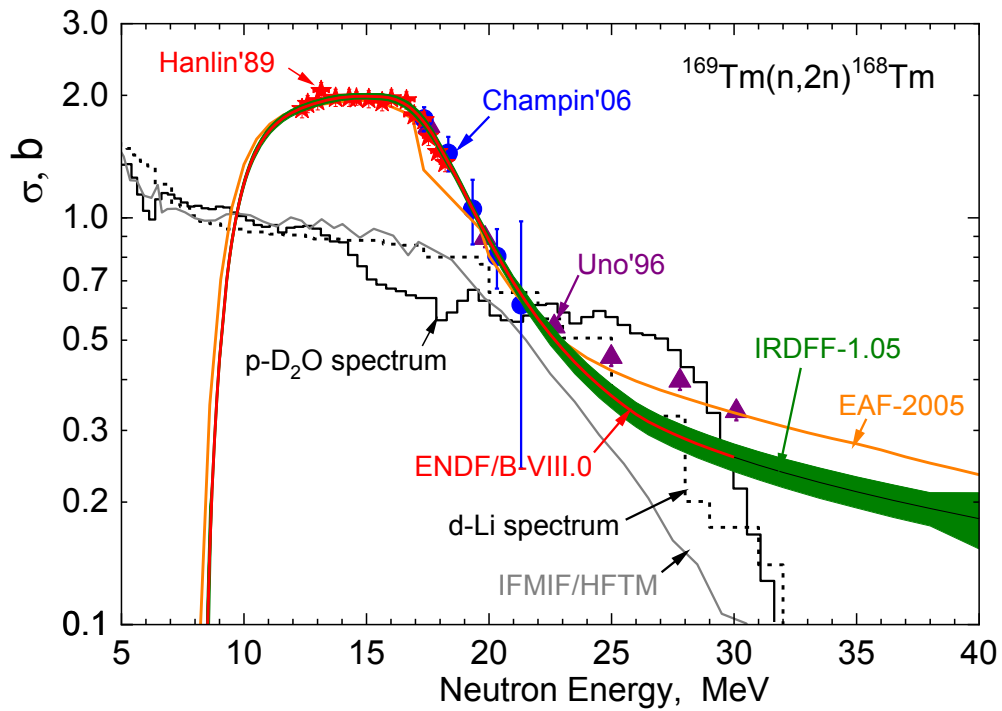
Fig. 1. ^{169}\text{Tm}(n,2n)^{168}\text{Tm} reaction cross sections
