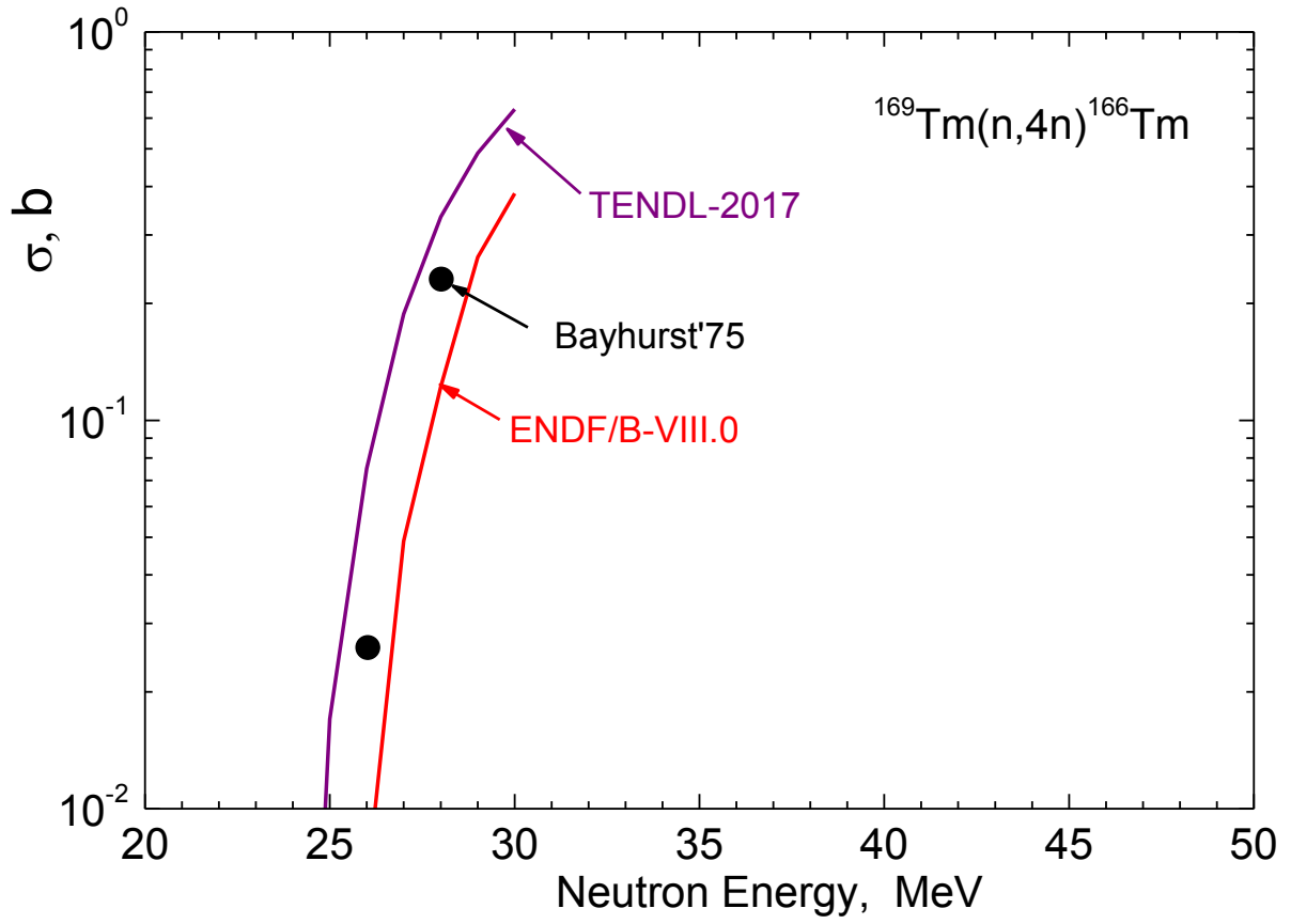
Fig. 3. ^{169}\text{Tm}(n,4n)^{166}\text{Tm} reaction cross sections
