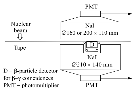
Fig. 1. Scheme of the total absorption spectrometer
