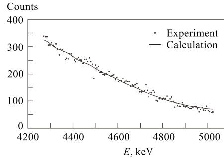
Fig. 4. Experimental and calculated TAS \gamma spectra for ^{156}\text{Ho} \beta^+ /EC decay in the analyzed interval
