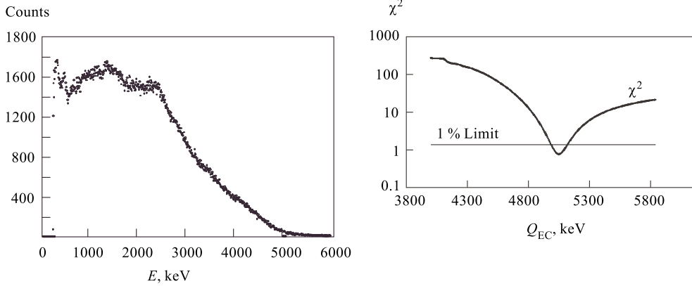
Fig. 2. Experimental TAS \gamma spectrum for ^{156}\text{Ho} \beta^+ /EC decay
