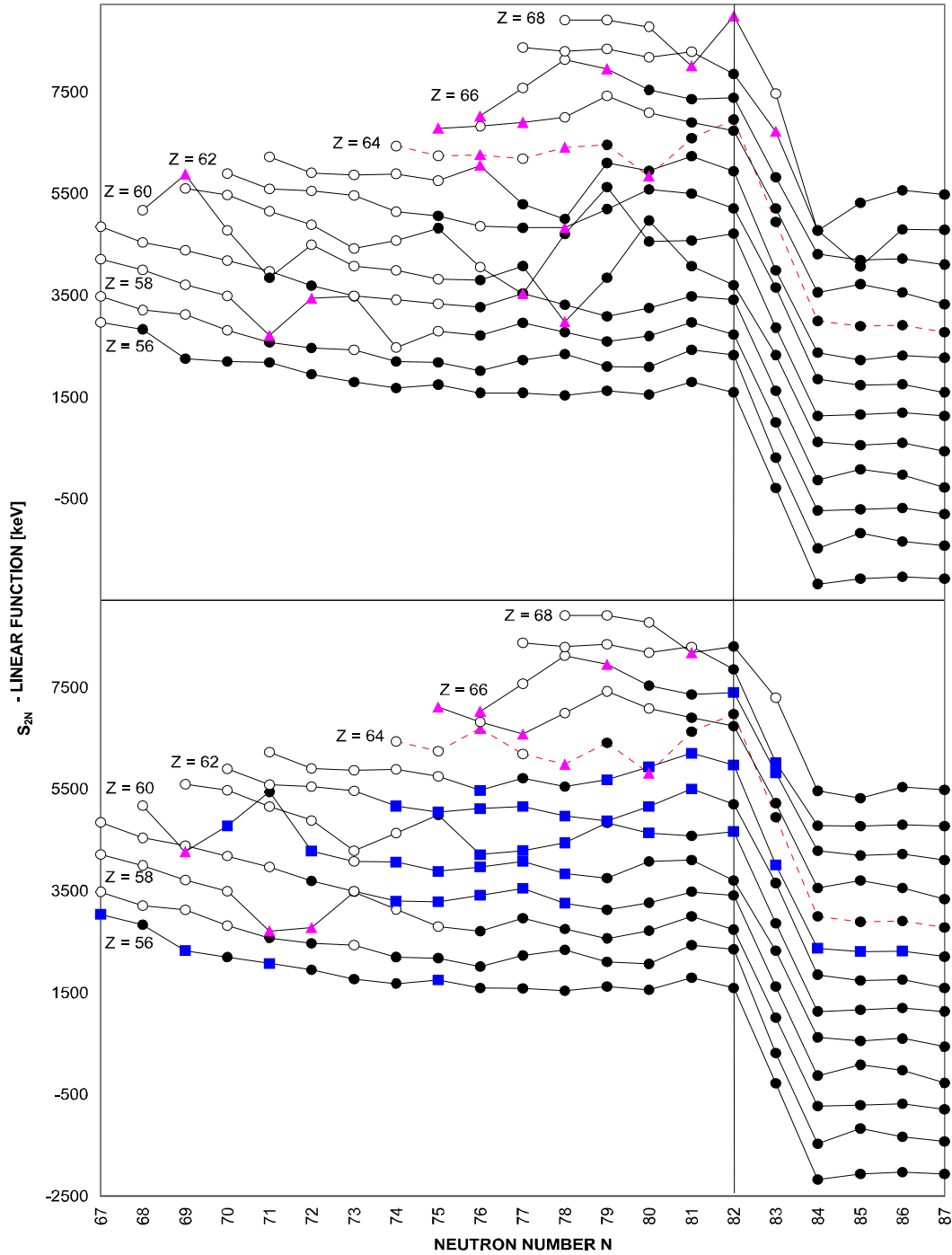
Fig. 9. Two-neutron separation energies as a function of neutron number for different nuclides. Shown are the values without (top) and including (bottom) the ISOLTRAP data. The nuclides are marked by squares (mass values measured by ISOLTRAP), solid circles (other experimental mass values), open circles (mass values estimated from systematic trends) and triangles (doubtful experimental value [27]).
