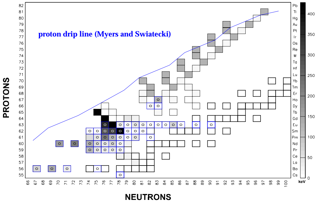
Fig. 5. Result of the far-reaching influence for ISOLTRAP data on the atomic mass evaluation. Shown is the change of the mass values after the Penning trap data have been added to the other input data of the AME95 [27]. The nuclides measured by ISOLTRAP in this work are marked by a circle. Stable nuclides are surrounded by thick lines. The proton drip line is indicated as calculated by Myers and Swiatecki [28].
