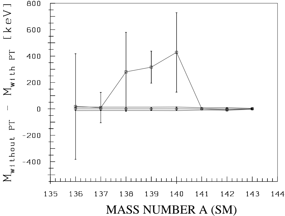
Fig. 6. Difference between the ISOLTRAP results (circles with error band) and the values from the 1995 atomic mass evaluation excluding the ISOLTRAP data (squares with error bars) for the samarium isotopes with 136 \leq A \leq 143 . The solid line through the 1995 values excluding the ISOLTRAP data serves only to guide the eye.
