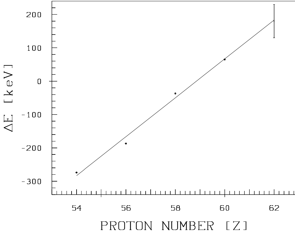
Fig. C.1. Energy differences between the I = 9/2^- and the I = 1/2^+ states of some even-odd nuclei along the N = 75 line. The energy difference for ^{137m}\text{Sm} ( Z = 62 ) is extrapolated. The solid line is a fit of a linear function through the data points.
