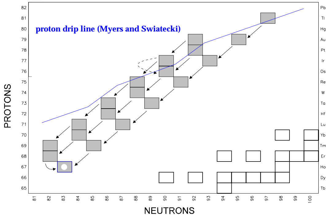
Fig. 7. Connection between mass values around ^{150}\text{Ho} (indicated, by a white circle). The connections shown are Q_\alpha -measurements (solid straight lines), one Q_\beta -measurement (solid curved arrow) and a Q_p -measurement of ^{167}\text{Ir} (dashed curved arrow). Stable nuclides are marked by white squares. The proton drip line is indicated as calculated in [28].
