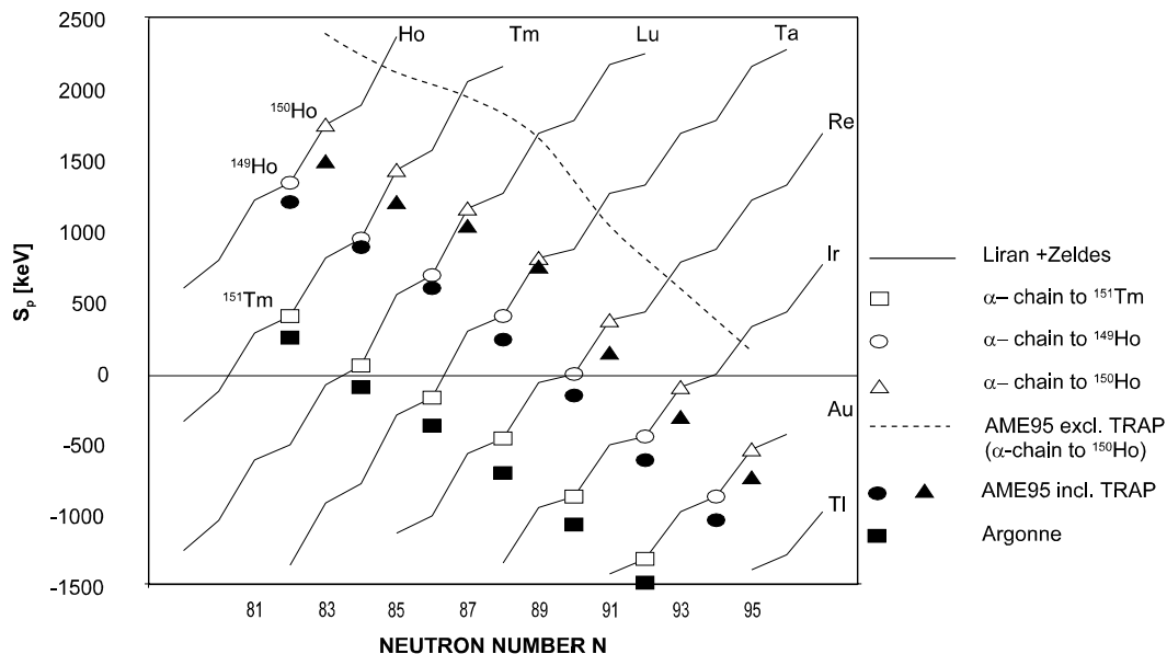
Fig. 10. Proton separation energies as a function of neutron number for different elements. The individual \alpha -decay chains are marked by squares (endpoint ^{151}\text{Tm} ), circles (endpoint ^{149}\text{Ho} ) and triangles (endpoint ^{150}\text{Ho} ). The open symbols on the black lines indicate the values predicted by Liran and Zeldes [39]. Filled symbols indicate the \alpha -chains after the ISOLTRAP data has been added to the atomic mass evaluation 1995. To demonstrate the influence of the ISOLTRAP data, the dashed line indicates the \alpha -decay chain to ^{150}\text{Ho} derived from an earlier experimental mass value of this nuclide.
