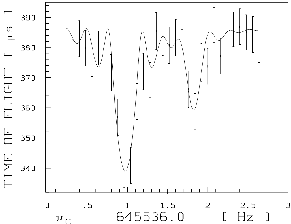
Fig. 4. Cyclotron resonances of ^{141}\text{Sm} ions in the isomeric (left) and ground state (right). Both species were stored simultaneously in the trap. From the center frequencies of the resonance curve the excitation energy of the isomer can be determined with \Delta E = 171(4) keV. The solid line is a fit of the theoretical line shape to the data points.
