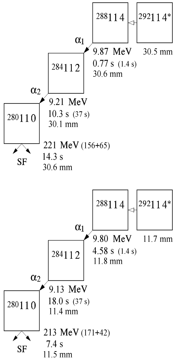
Fig. 1. Time sequences in the observed decay chains. The expected half-lives corresponding to the measured E_\alpha values for the given isotopes are shown in parentheses following the measured lifetimes. Positions of the observed decay events are given with respect to the top of the strip.
