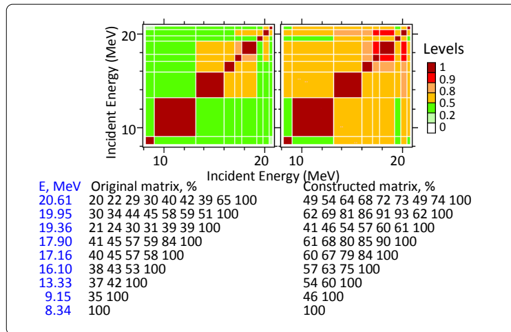
Fig. 1. Experimental (left) and constructed correlation matrices using only C5 (right)
