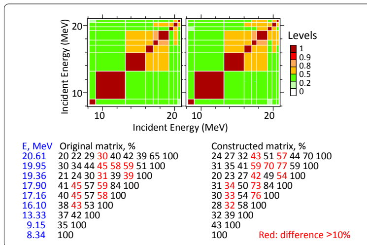
Fig. 2. Experimental (left) and constructed correlation matrices using C5 and MERC defaults (right)
