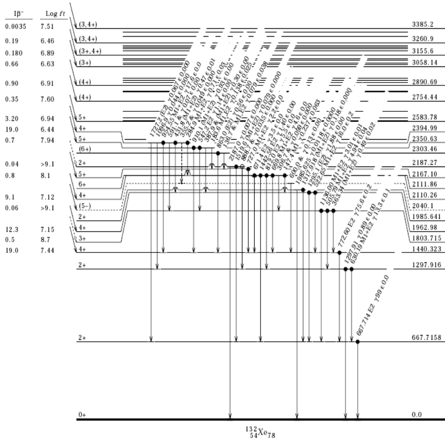
Fig.5 Decay Scheme of ^{132}\text{I} (partial)
