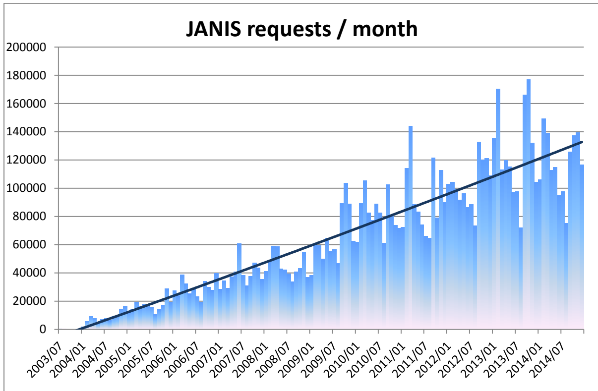
Figure. Number of requests per month to the remote JANIS database since 2003.
